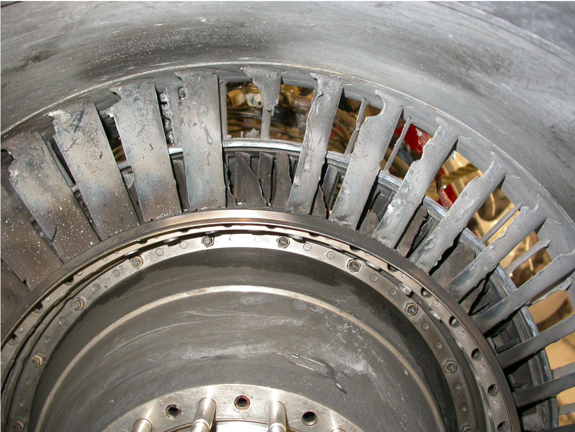
View of fractured and damaged stator vanes.
