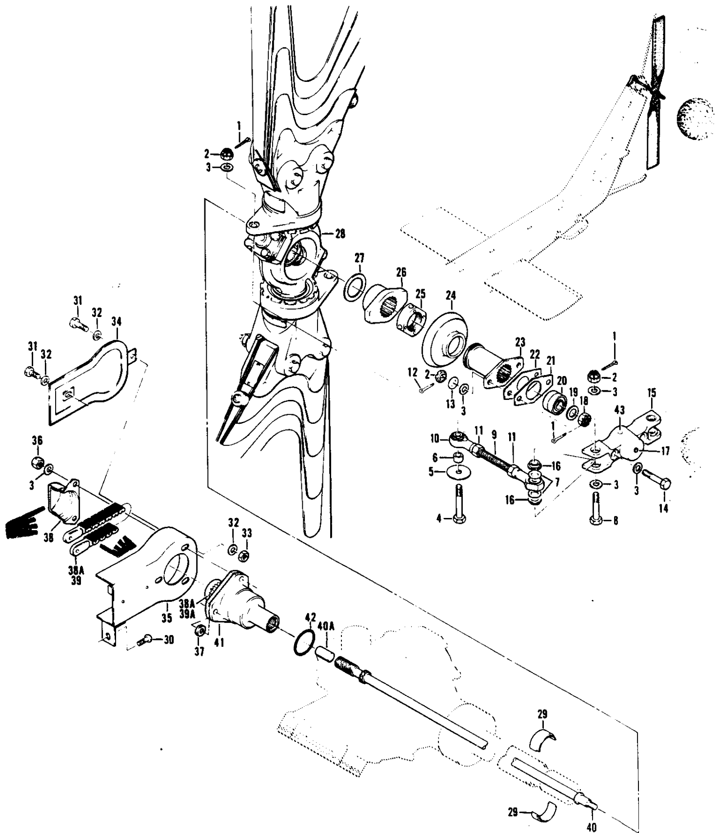
Figure 145. Tail Rotor Installation
