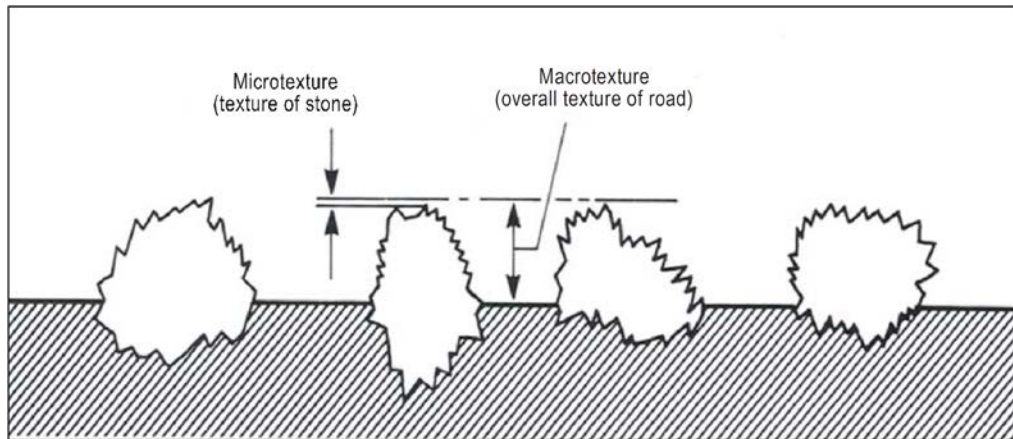
Figure 11 – Pavement texture (ref. 14)
