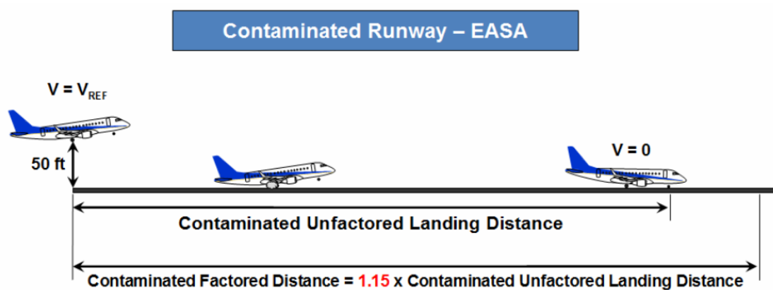
Figure 6 – Contaminated factored landing distance (EASA)
