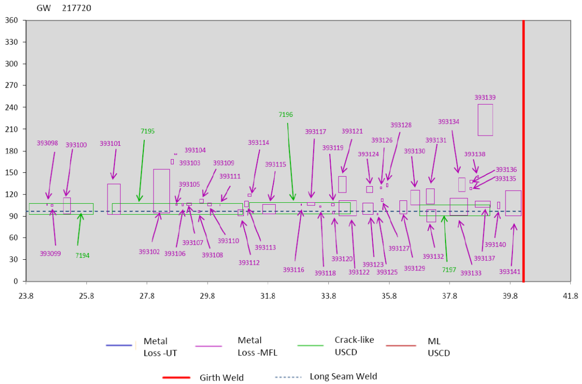
Figure 6: Summary of MFL and USCD ILI data for the ruptured pipe joint (part 2/2) provided by Enbridge.
