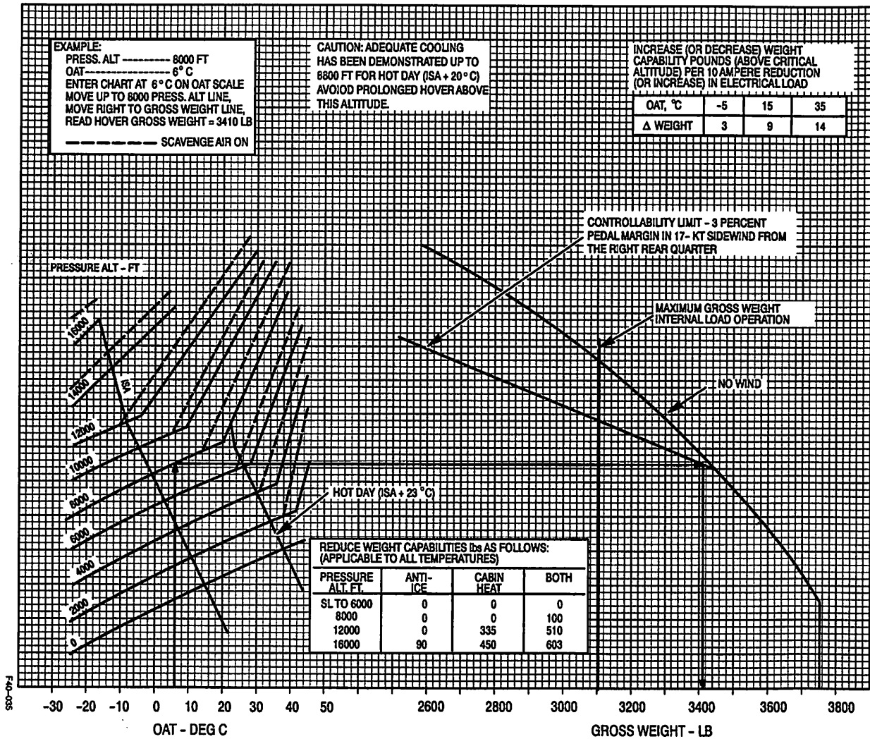
Figure 8-2. Hover Ceiling, OGE, Engine Air Particle Separator Inlet
