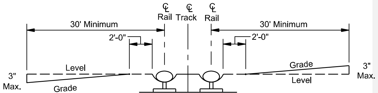
PROFILE AT RAILROAD/HIGHWAY GRADE CROSSINGS
