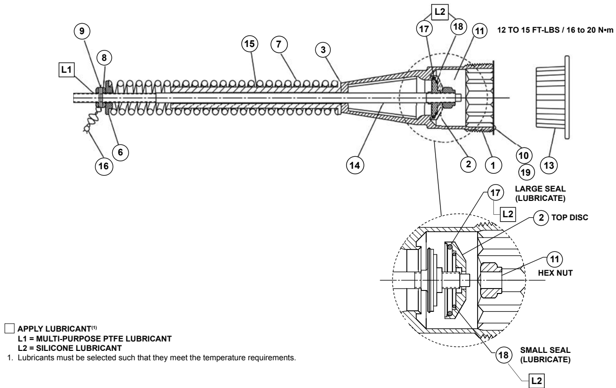
Figure 4. Types H732A and H832A Relief Valves
