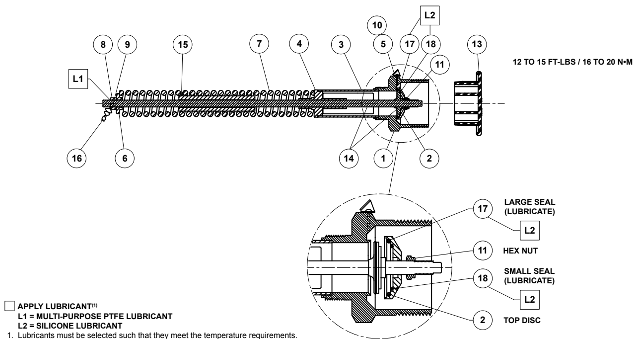
Figure 5. Types H282, H882, H5112 and H8112 Relief Valves
