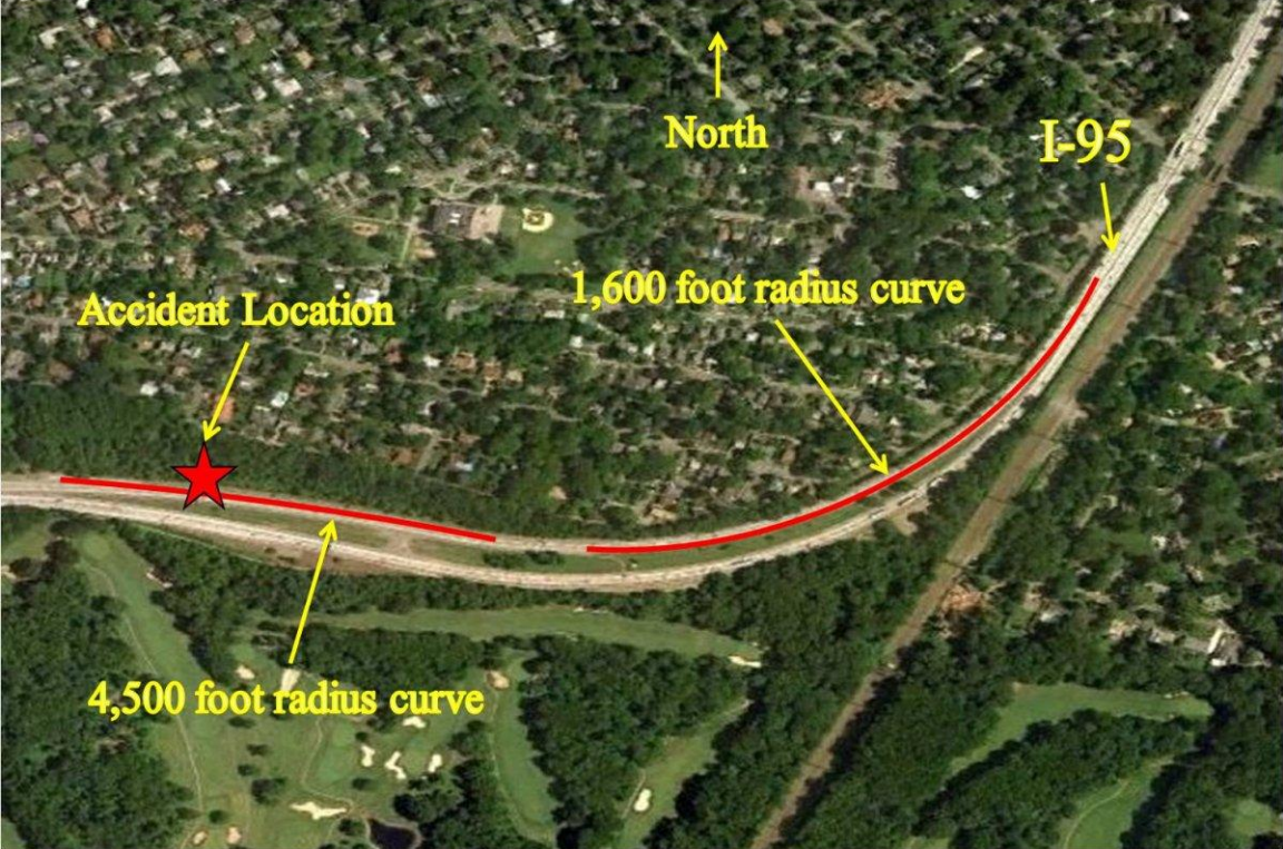
HWY Photo-02, Illustrating the 1,600 foot radius and 4,500 foot radius horizontal curves
