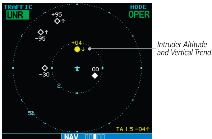
Figure 5 Intruder Altitude and Vertical Trend Arrow
