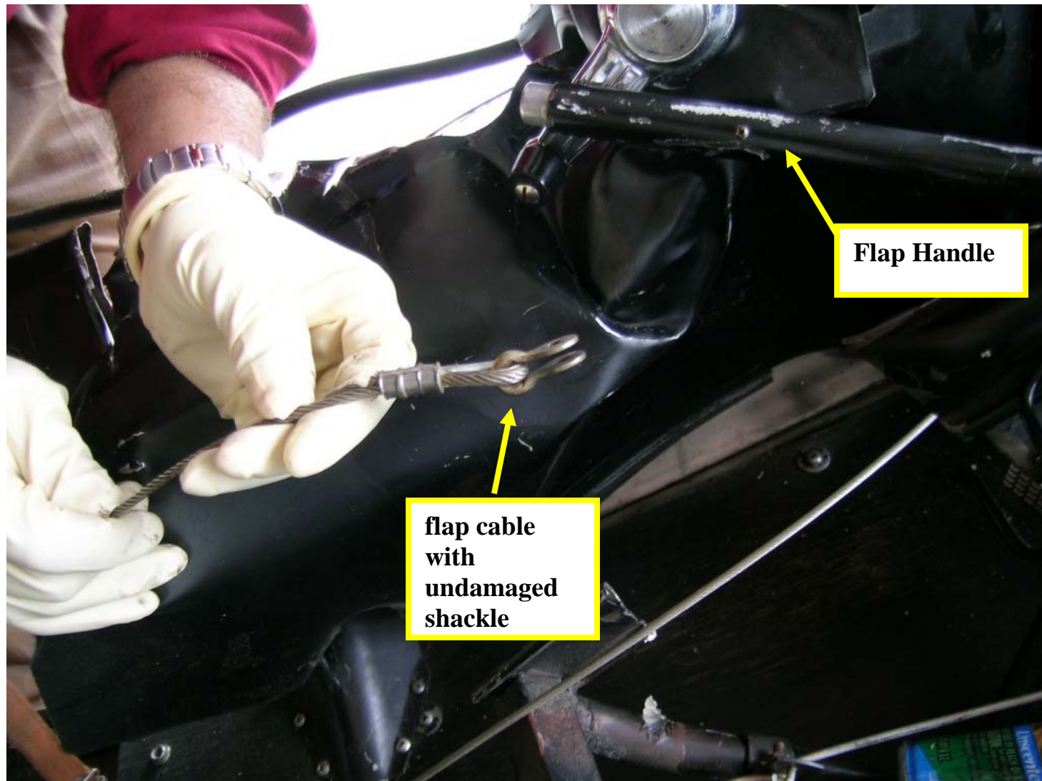
Fig 3 - Flap Cable with Undamaged Shackle
