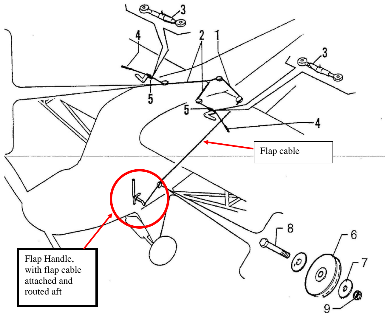
Fig 1 - General Arrangement, Flap Handle and Cable
