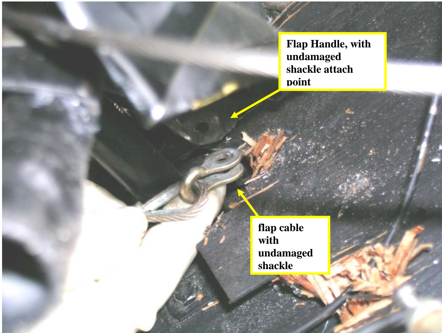
Fig 4 - Flap Cable with Undamaged Shackle and Handle Attach Point
