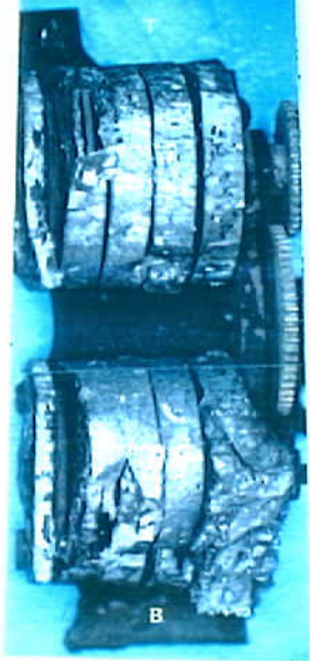
Figure 2. Close View of the Fire Damage to the Front of the Drum Counters. (4X)
