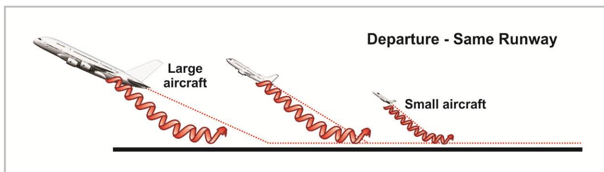
FIGURE 9. DEPARTING SAME RUNWAY BEHIND A LARGER AIRCRAFT
