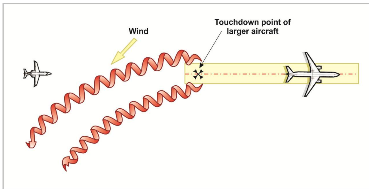
FIGURE 11. AVOIDANCE PROCEDURES LANDING BEHIND LARGER AIRCRAFT ON THE SAME RUNWAY
