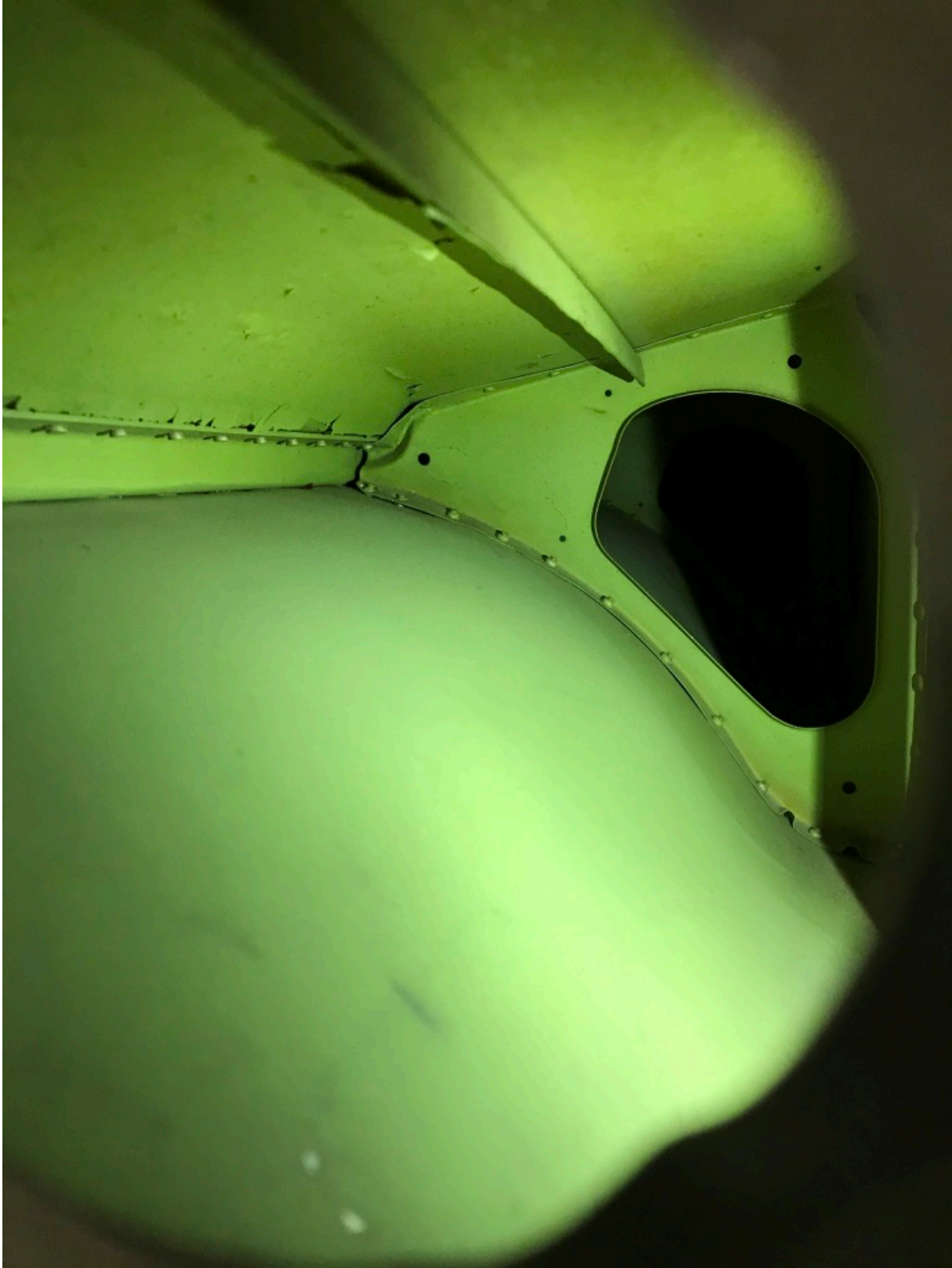
Figure 4 - Internal Rib Wrinkles
