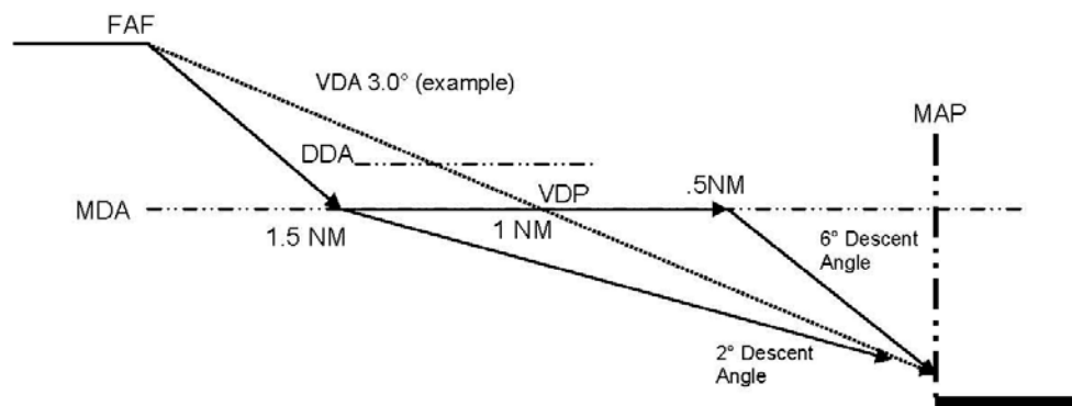
FIGURE 1A. APPROACH EXAMPLE WITHOUT USING CONTINUOUS DESCENT FINAL APPROACH
