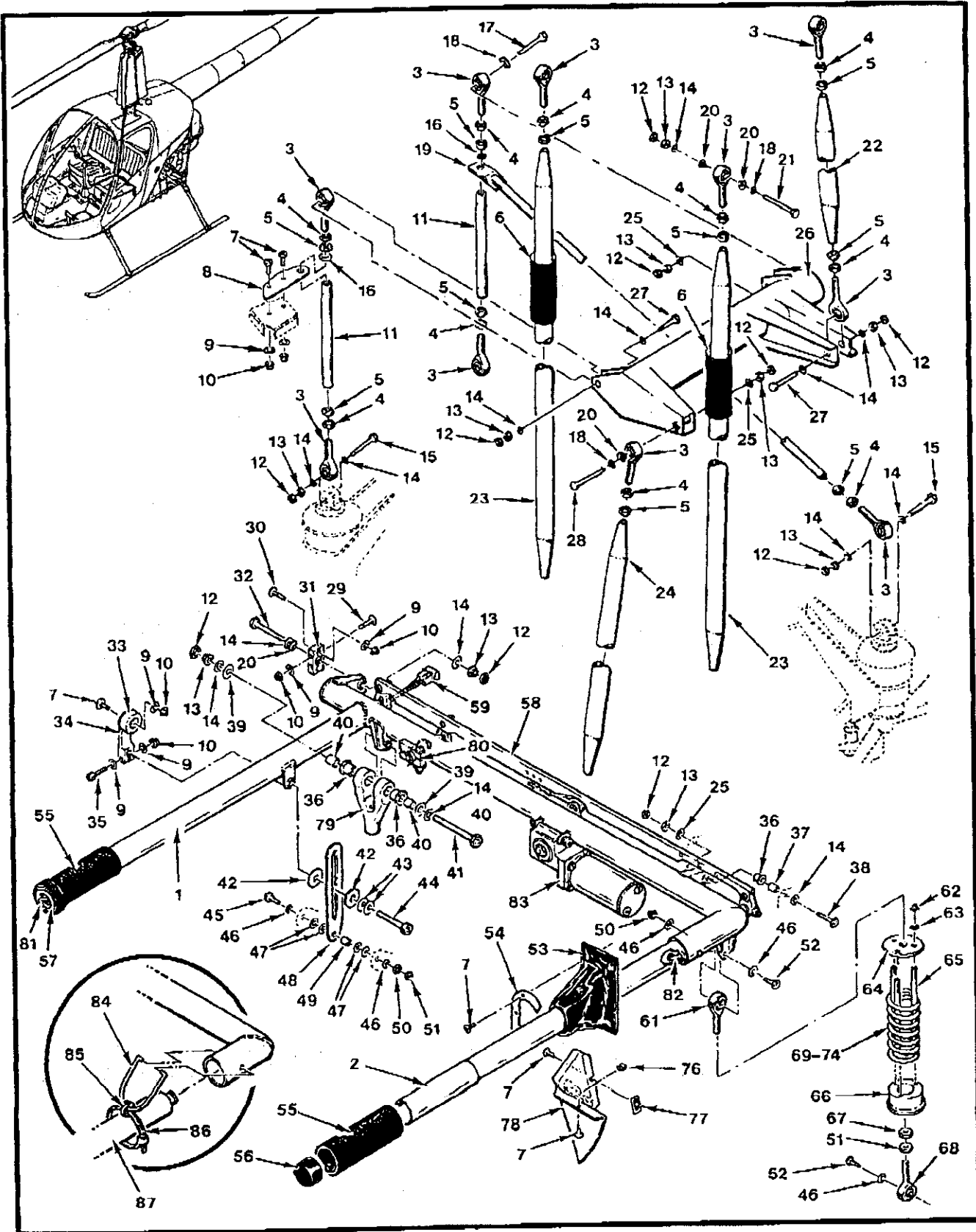
FIGURE 7-11 COLLECTIVE CONTROL SYSTEM
