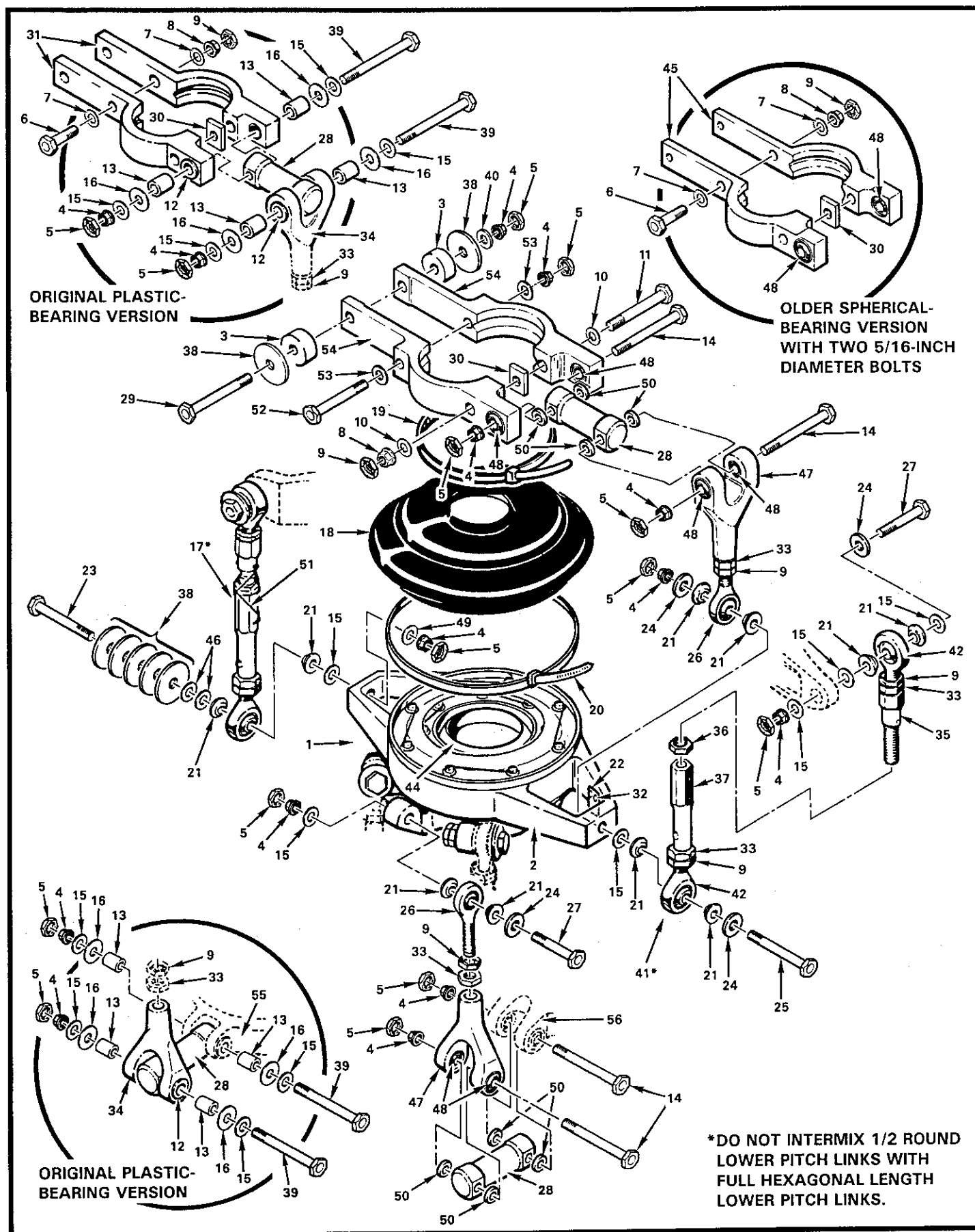
FIGURE 7-15 SWASHPLATE ASSEMBLY (Original equipment on Ship S/N 3539 and prior)
