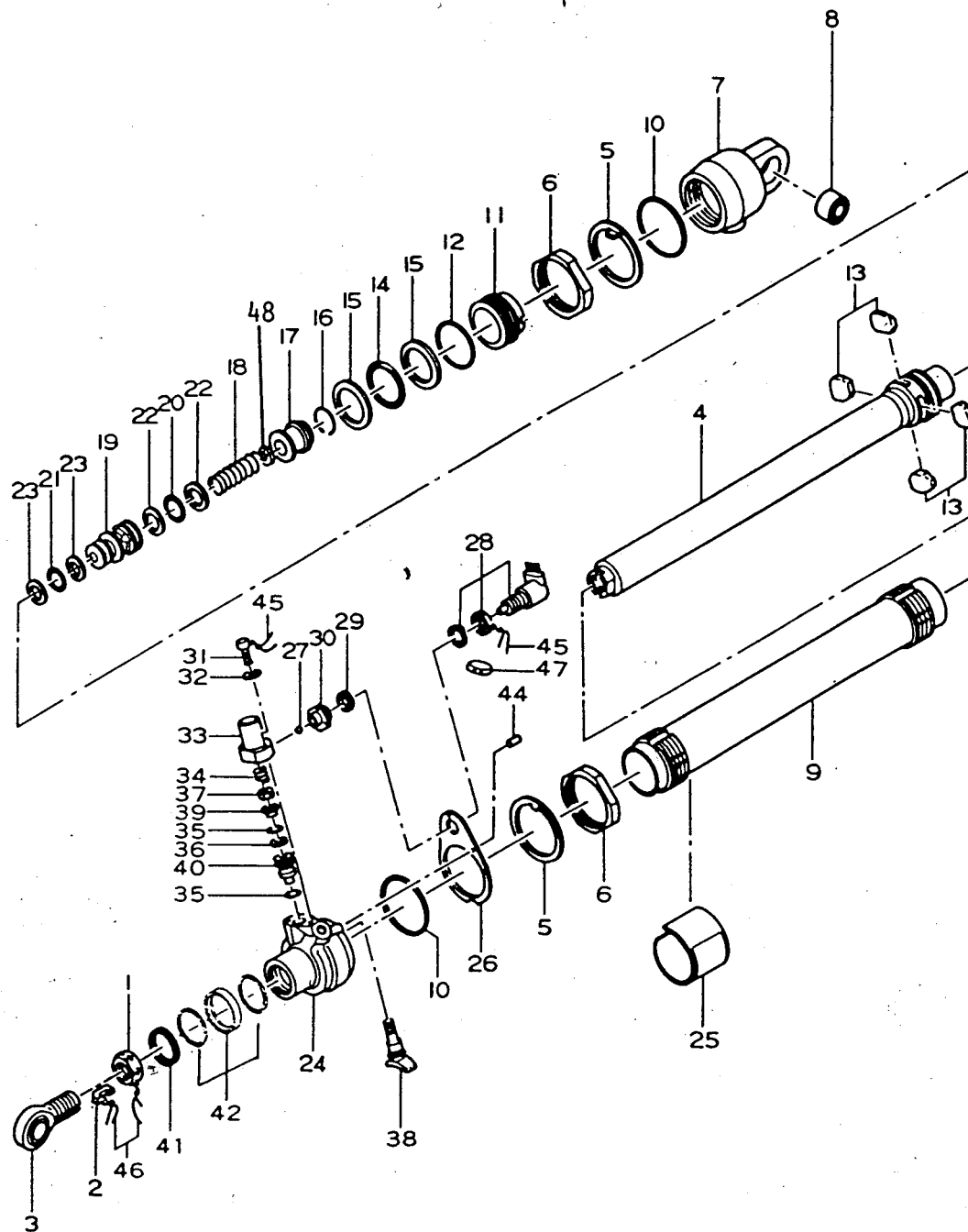
Fig. 1001 Actuator Assembly-MLG Hyd. Locking P/N 9910136-3 (Teijin Seiki P/N 1521200-5) P/N 9910136-4 (Teijin Seiki P/N 1521200-6) P/N 9910136-5 (Teijin Seiki P/N 1521200-7) P/N 9910136-8 (Teijin Seiki P/N 1521200-9) P/N 9910136-9 (Teijin Seiki P/N 1521200-10) P/N 9910136-10 (Teijin Seiki P/N 1521200-11)
