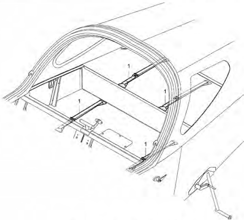
Figure 25-50-01, Fastening Straps Installation
