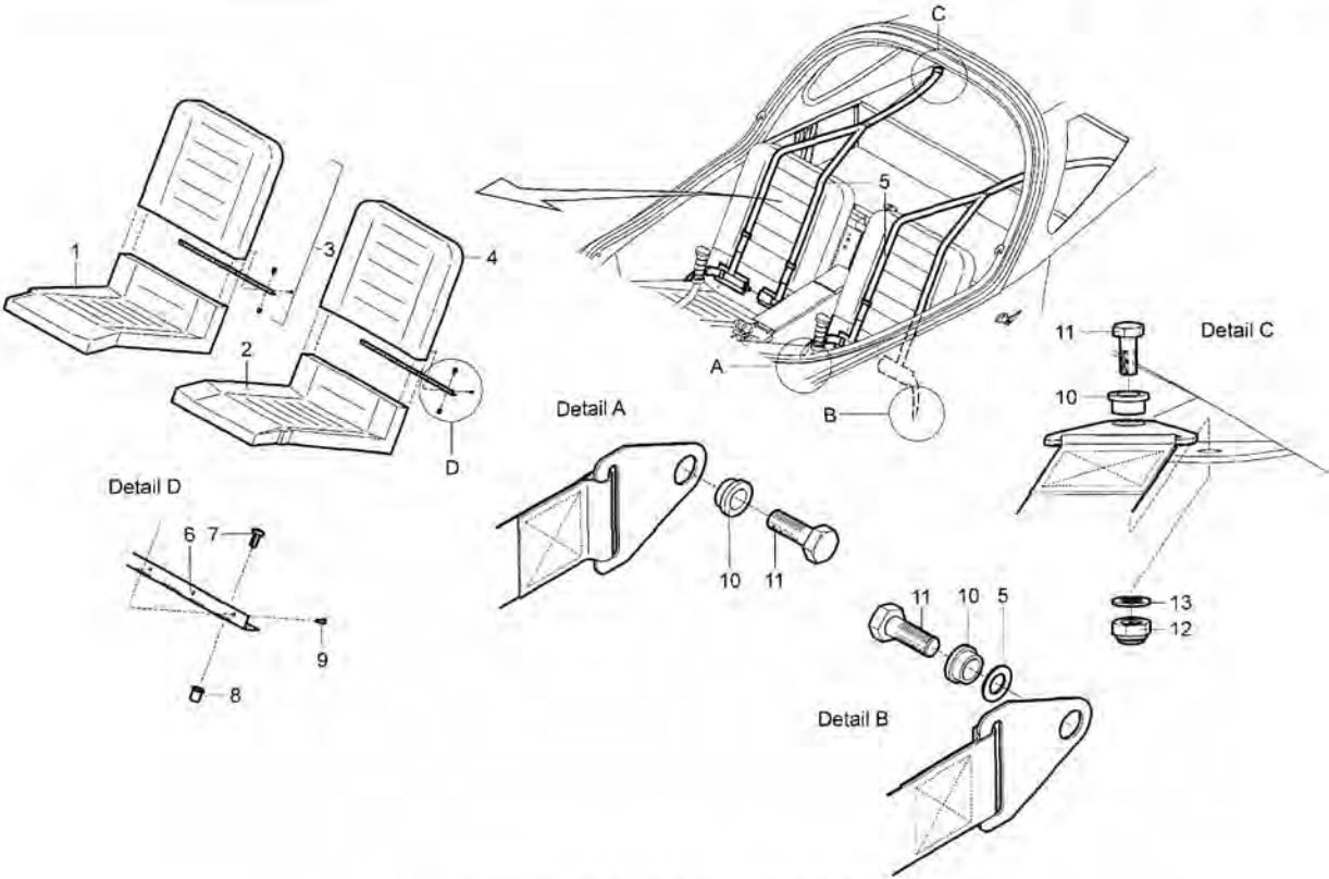
Figure 25-10-01, Upholstery Installation
