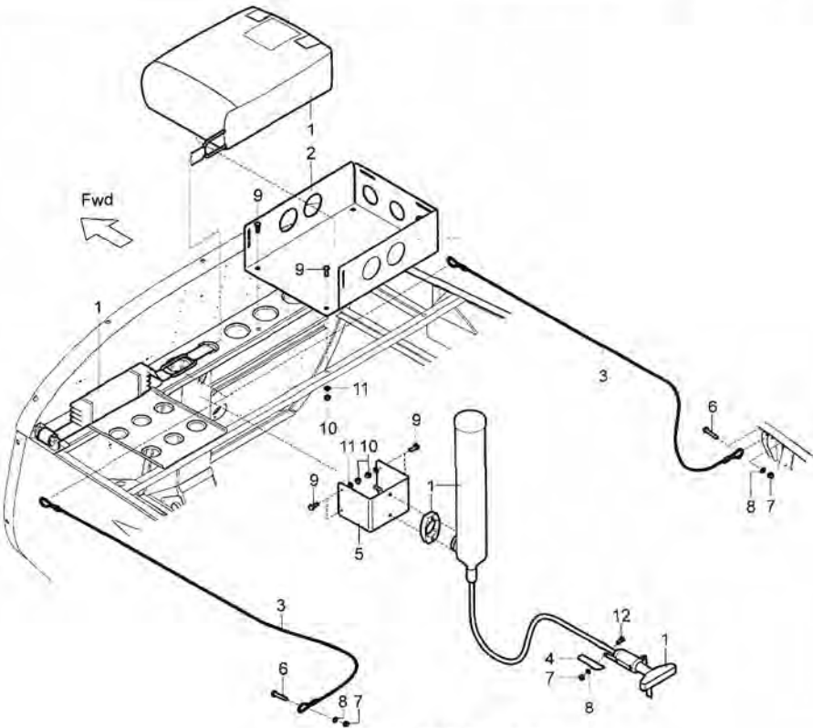
Figure 25-60-01, BRS Installation
