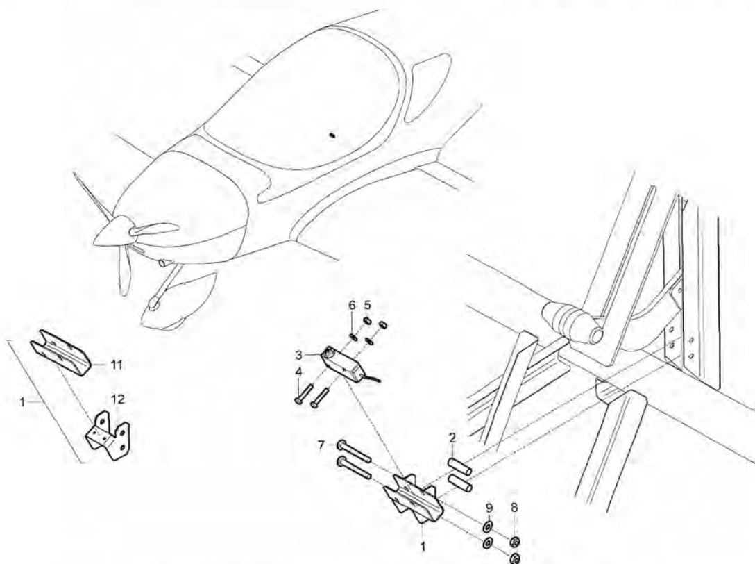
Figure 52-70-02, Control Lever Unlocked Micro Switch Installation
