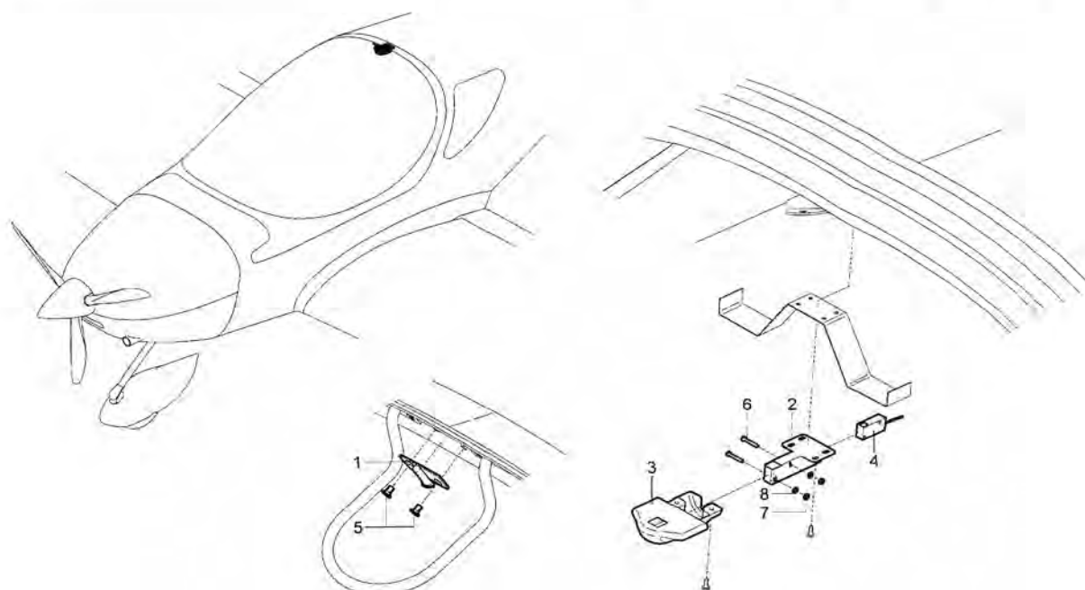
Figure 52-70-01, Canopy Unlocked Micro Switch Installation
