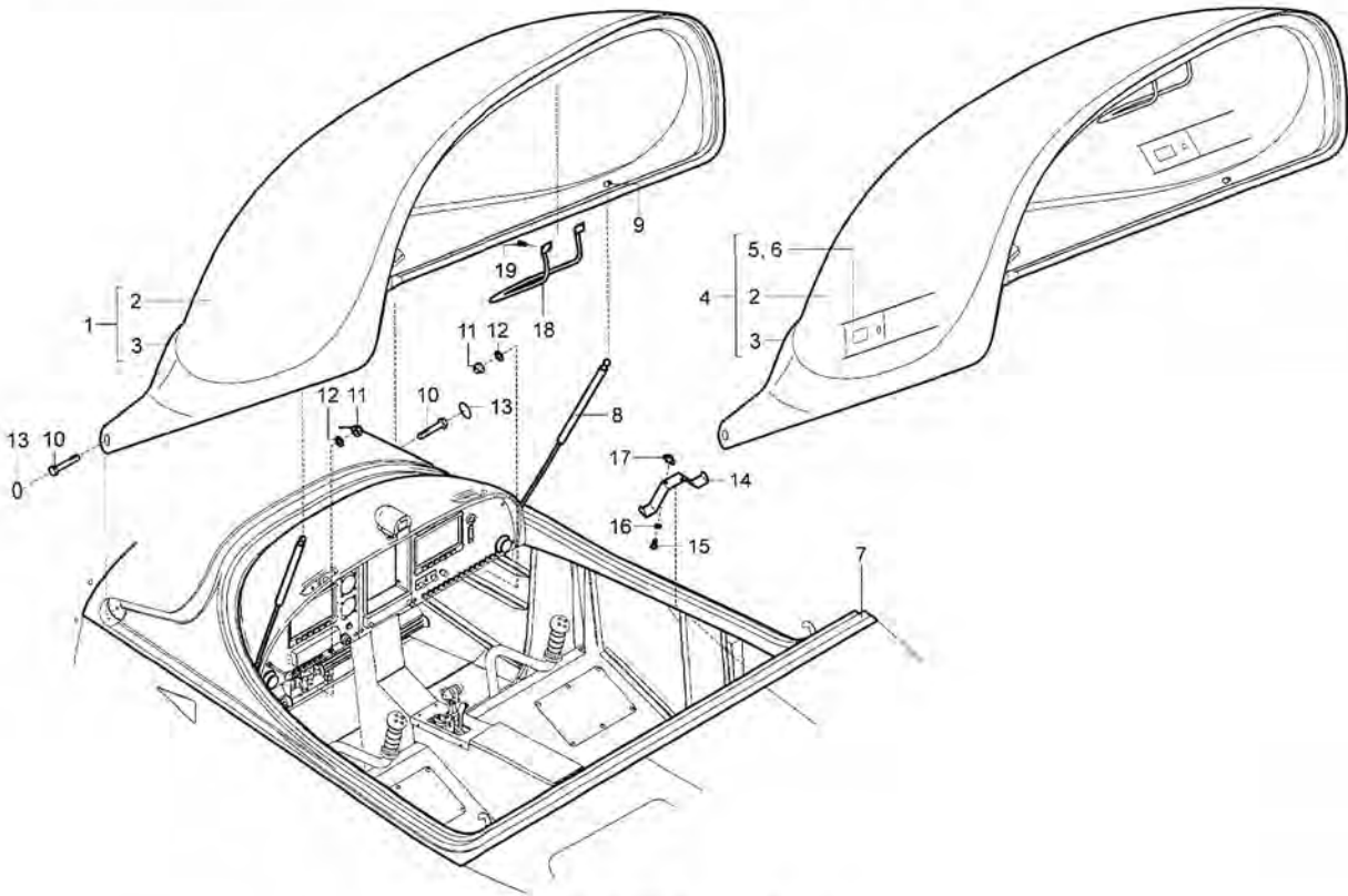
Figure 52-10-02, Canopy Door Assy
