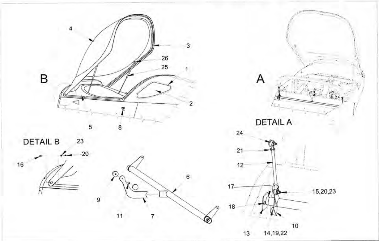
Figure 52-10-01, Canopy Door and Windows
