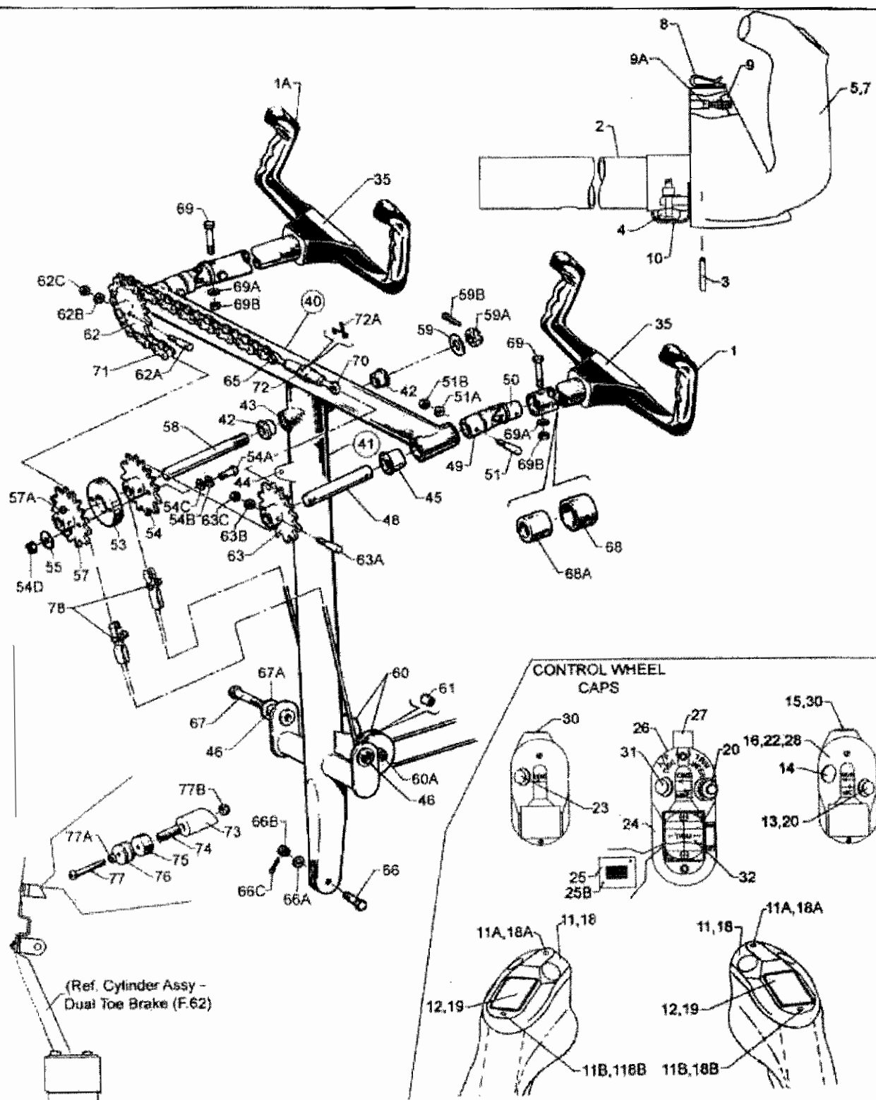
Figure 61. Control Wheel Installation
