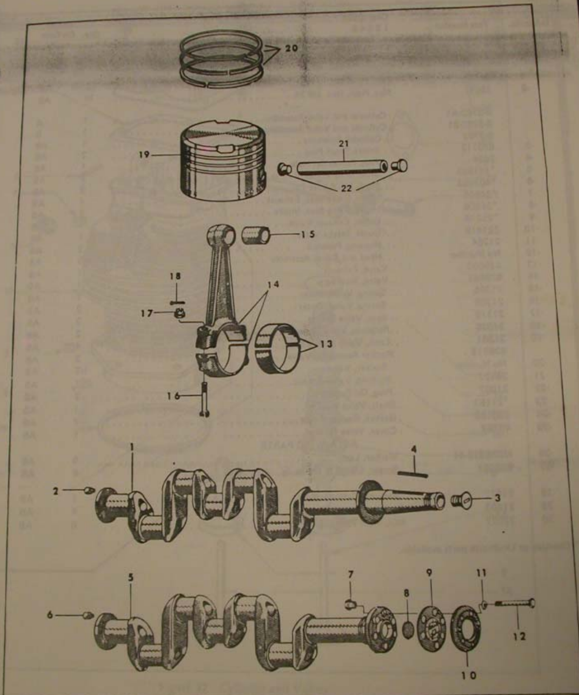
Figure 31. Crankshafts, Connecting Rods and Pistons.
