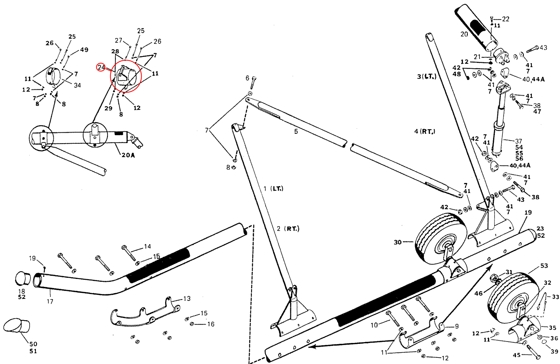
LANDING GEAR ASSEMBLY FIGURE 7-14
