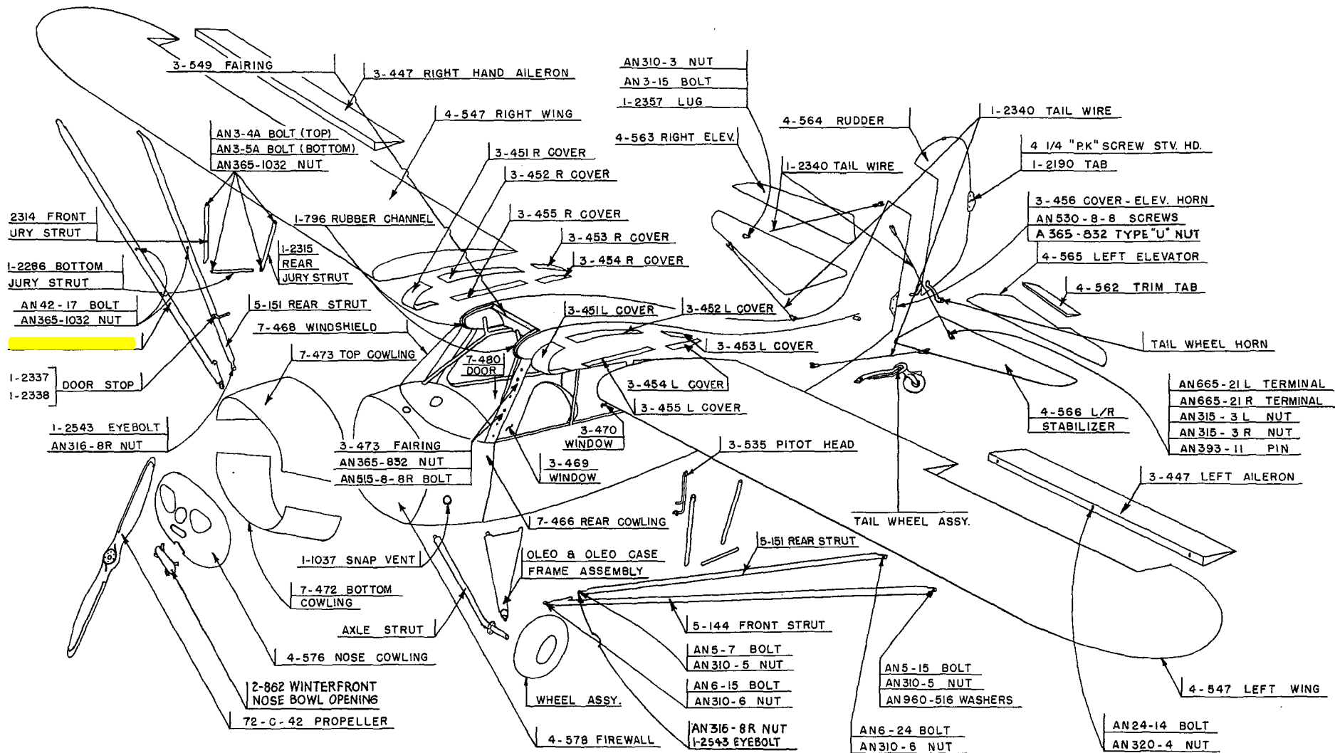
GENERAL EXPLOSION VIEW
