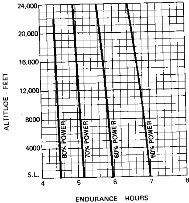
Figure 5-9. Endurance Profile
