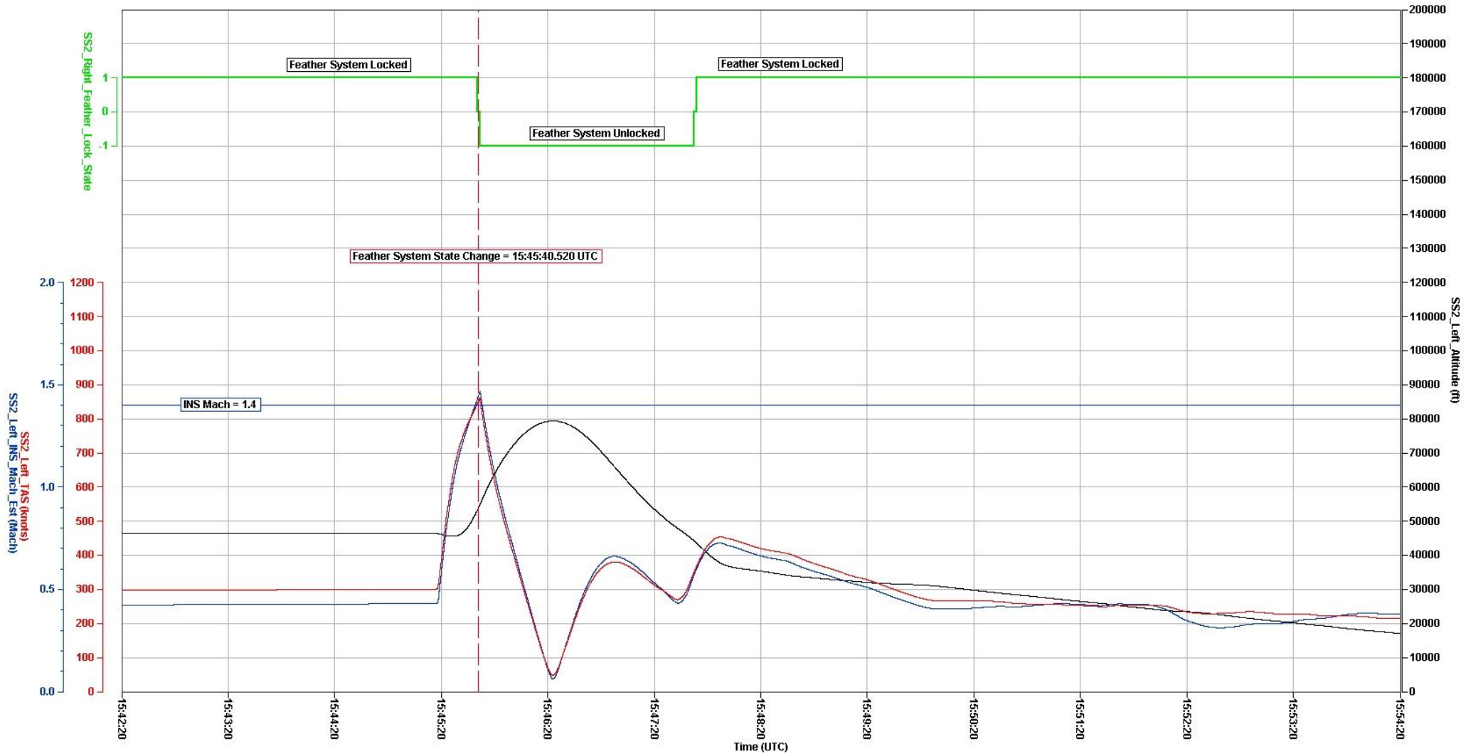
Figure 7. SIM SESSION 8 - RUN 002 Scaled Composites SpaceShipTwo, PF04-SIM8-002, N339SS
