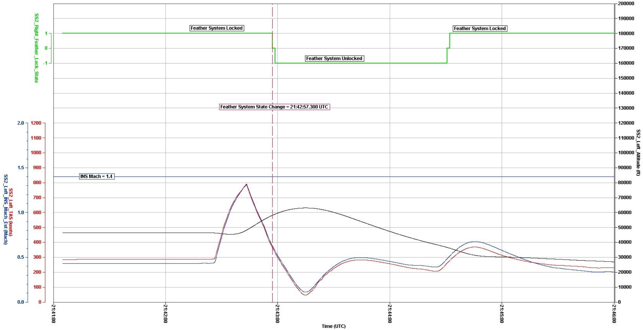
Figure 2. SIM SESSION 4 - RUN 003 Scaled Composites SpaceShipTwo, PF04-SIM4-003, N339SS
