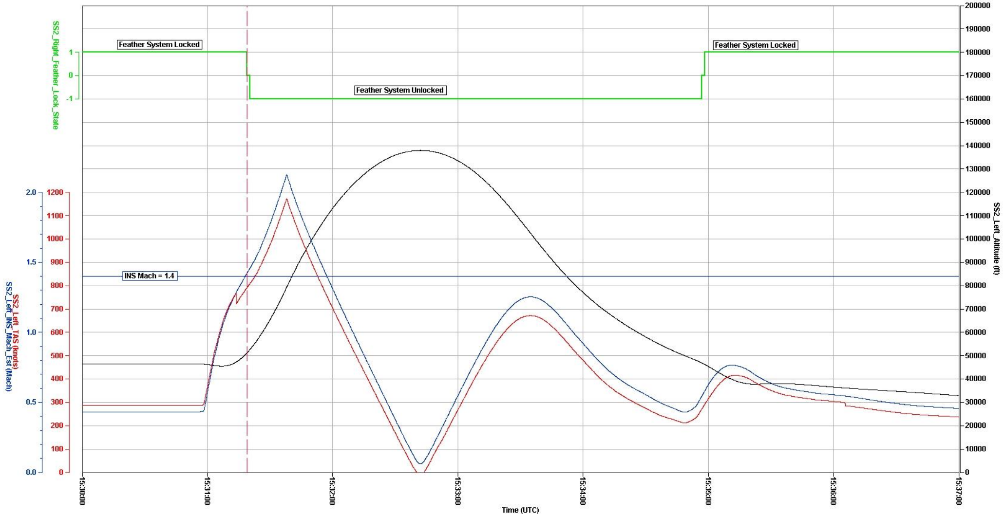
Figure 4. SIM SESSION 7 - RUN 002 Scaled Composites SpaceShipTwo, PF04-SIM7-002, N339SS
