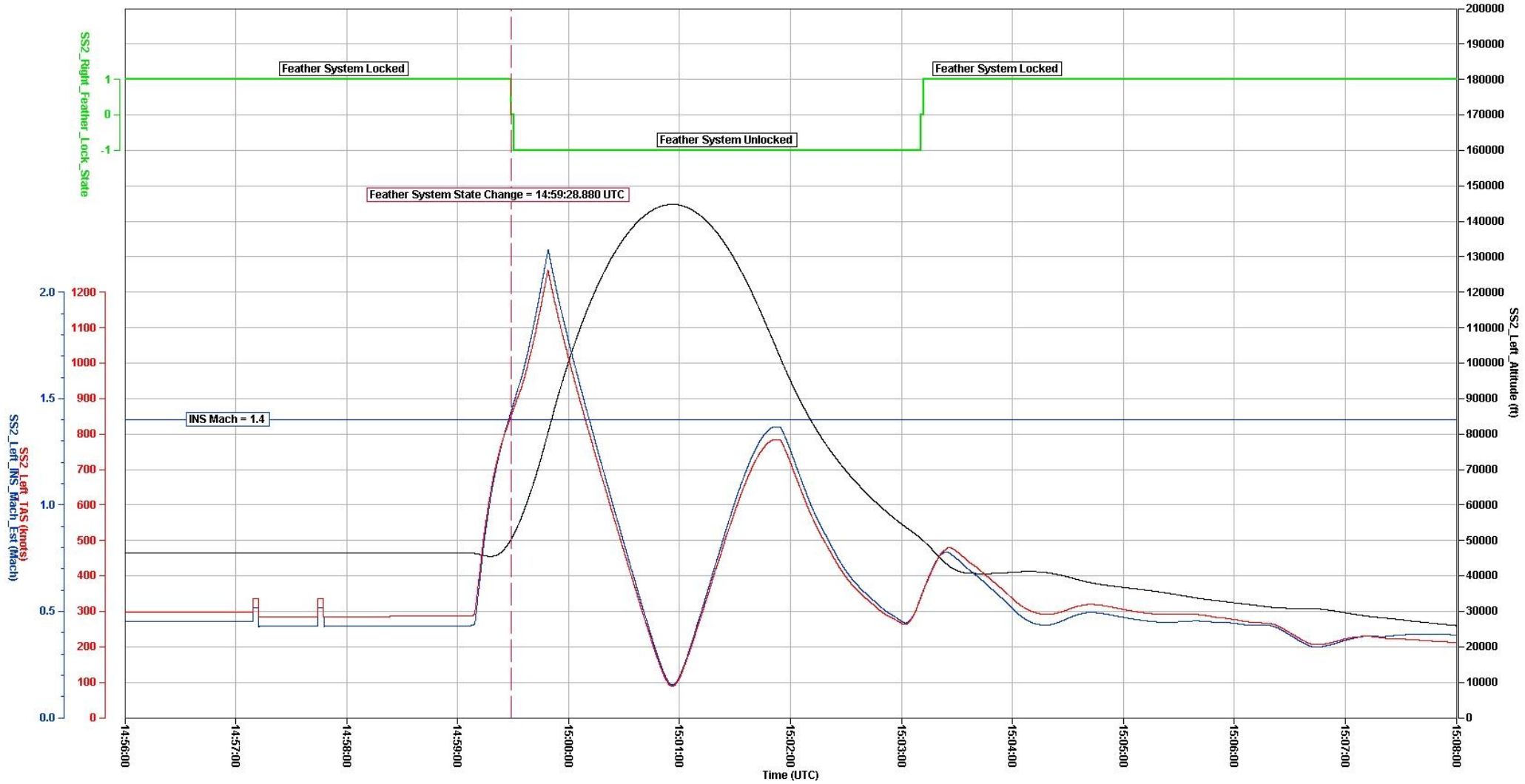
Figure 3. SIM SESSION 7 - RUN 001 Scaled Composites SpaceShipTwo, PF04-SIM7-001, N339SS
