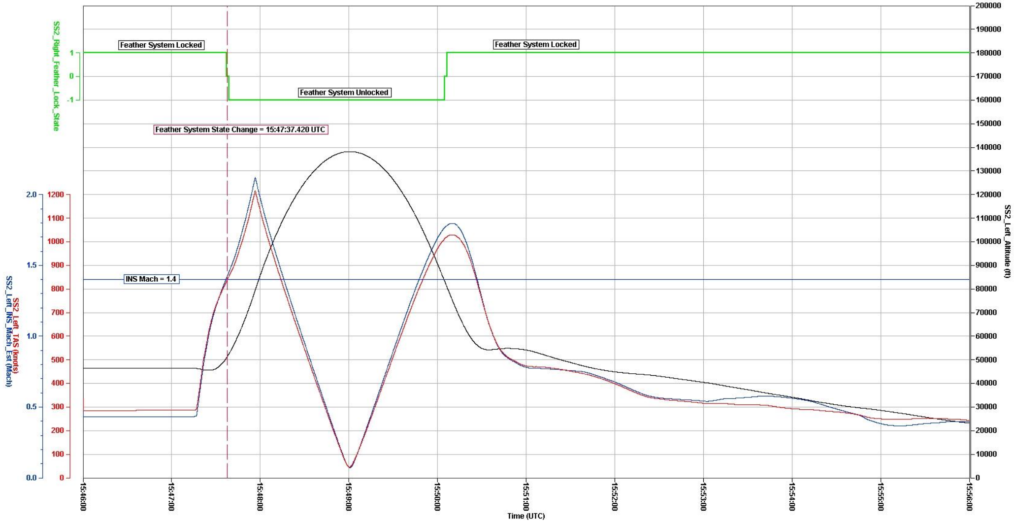
Figure 5. SIM SESSION 7 - RUN 003 Scaled Composites SpaceShipTwo, PF04-SIM7-003, N339SS
