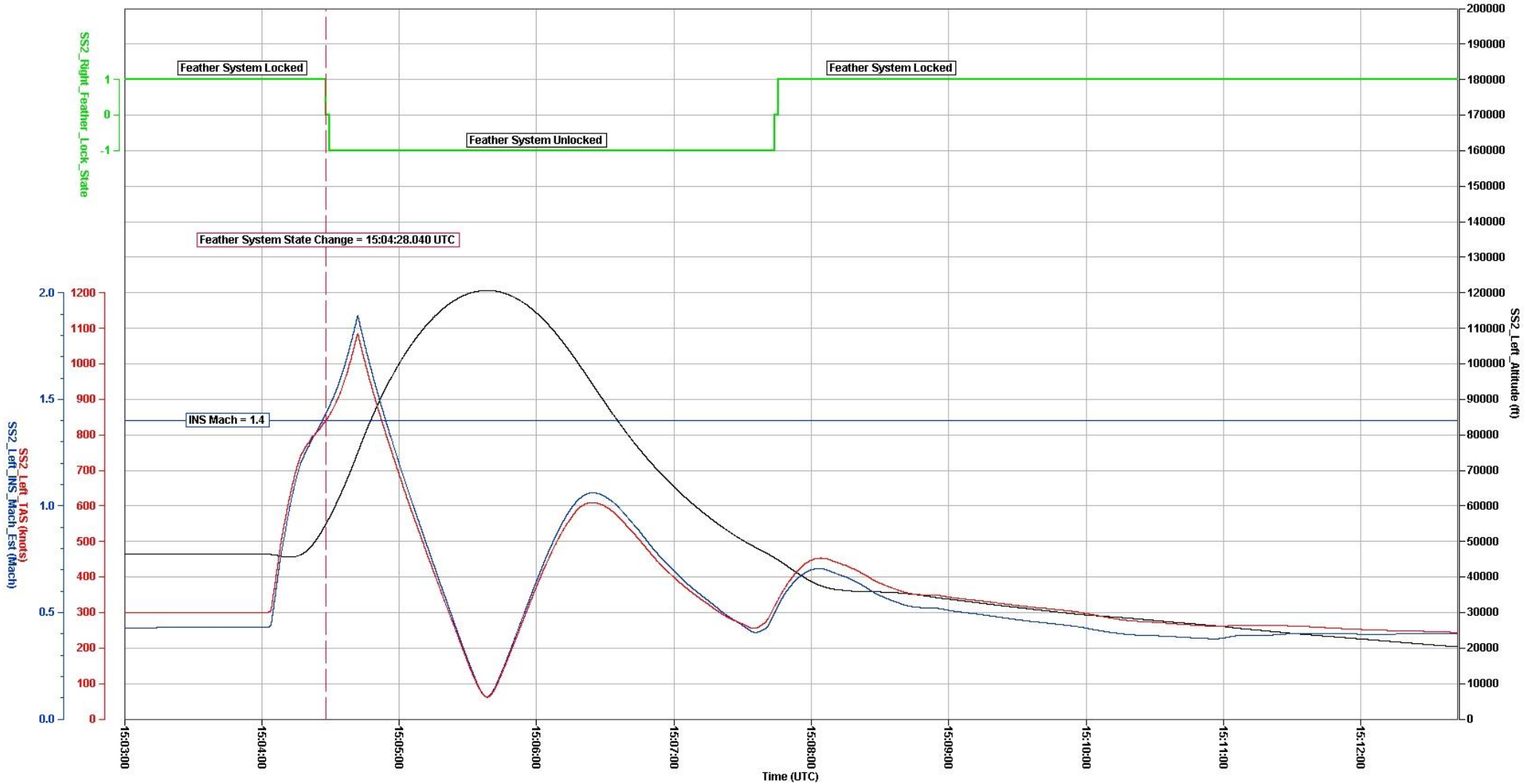
Figure 6. SIM SESSION 8 - RUN 001 Scaled Composites SpaceShipTwo, PF04-SIM8-001, N339SS
