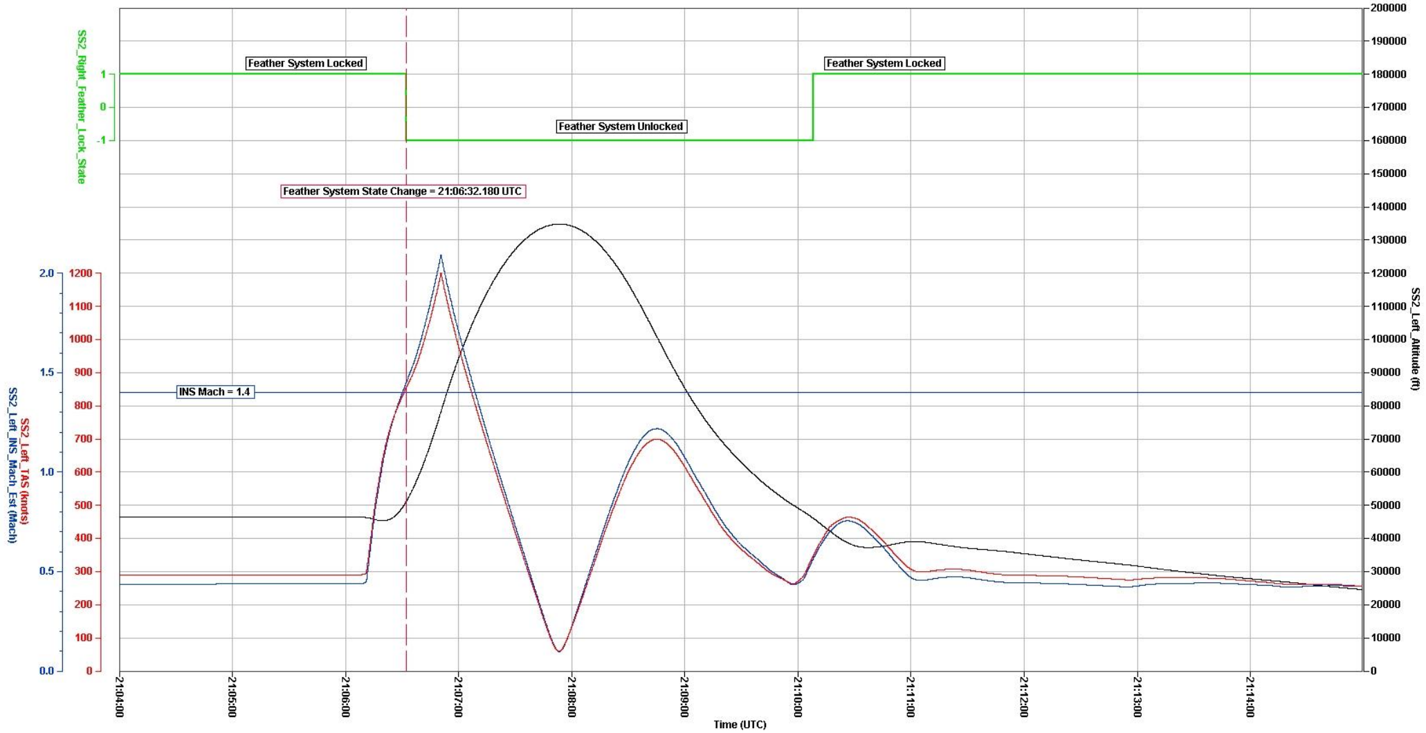
Figure 1. SIM SESSION 4 - RUN 001 Scaled Composites SpaceShipTwo, PF04-SIM4-001, N339SS
