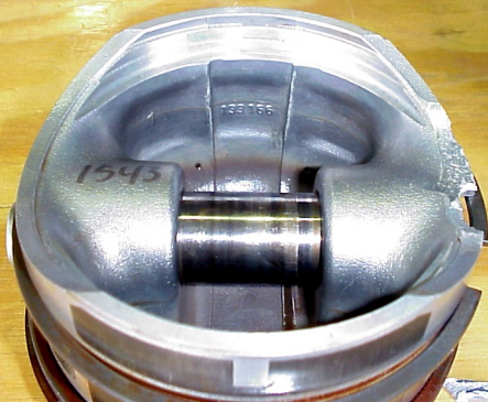
ECI Piston For Continental IO-550 Engine - Photo 7
