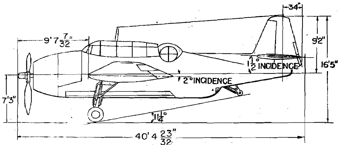
Figure 6 — Dimensional Diagram (Page 2 of 2 Pages)
