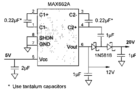
Figure 7—5V to 20V Converter
