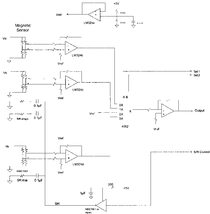
Figure 21—Three-Axis Low Cost Magnetic Sensor
