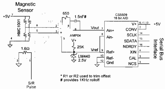
Figure 17—One-Axis Sensor With Digital Interface
