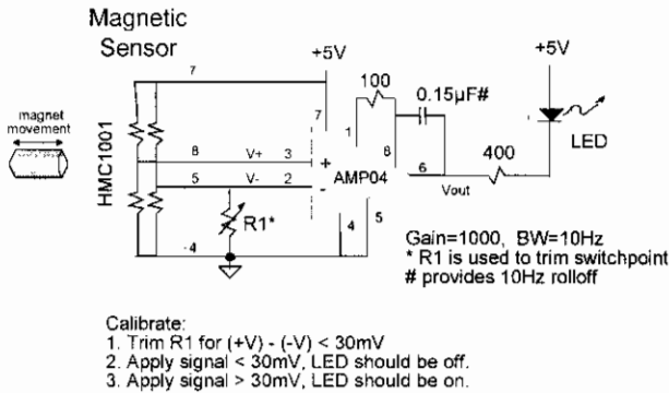
Figure 16—Magnetic Proximity Switch
