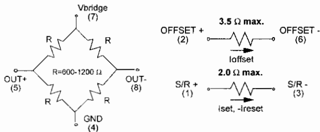
Figure 1—On-Chip components (HMC1001)
