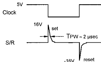
Figure 6—Single Clock Set/Reset Timing
