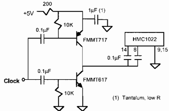
Figure 12—5V Circuit for SET/RESET (1021/1022)
