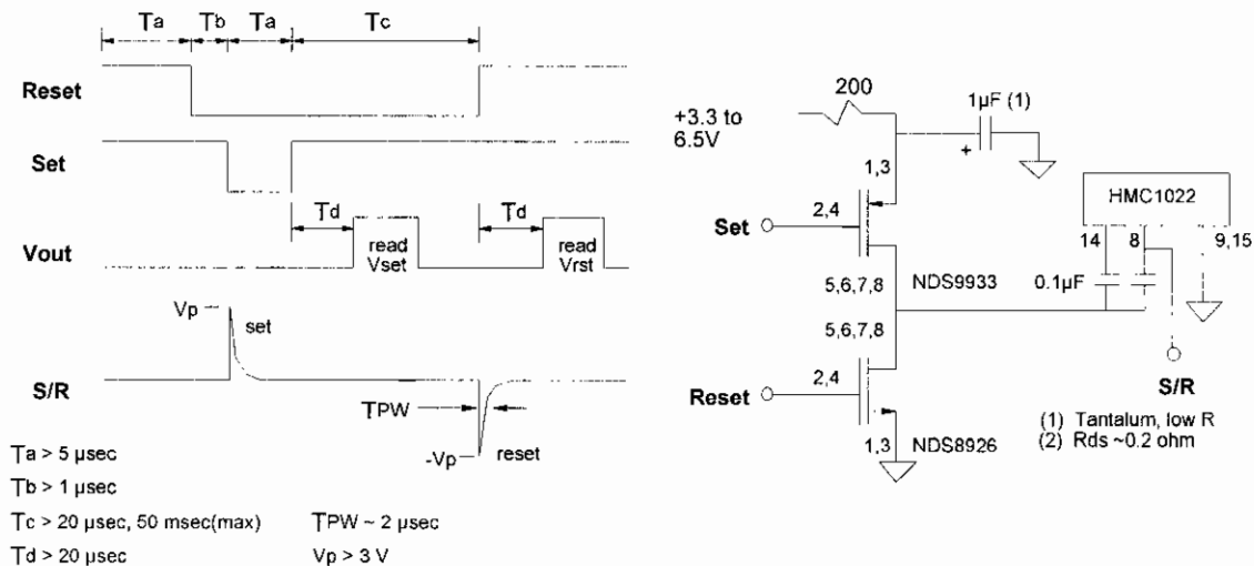
Figure 15—Single Clock Set/Reset Pulse Circuit (1021/1022)
