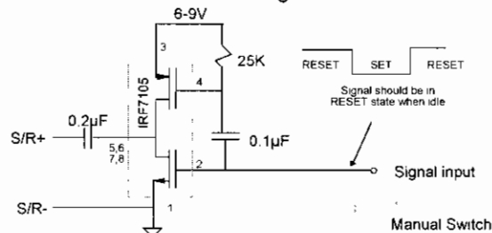
Figure 5—Single-Axis Set/Reset Pulse Circuit (1001)
