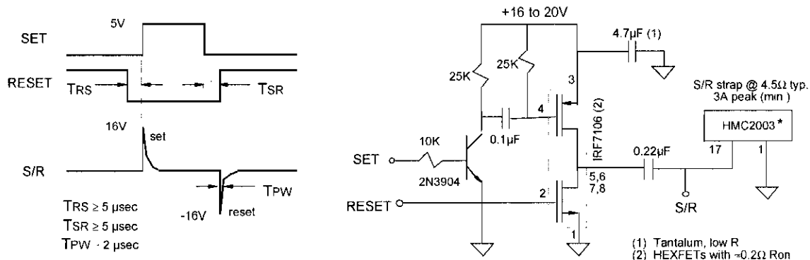
Figure 8—Single Clock Set/Reset Pulse Circuit (1001/1002)
