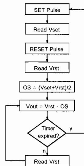
Figure 14—Low Power Set/Rst Flowchart
