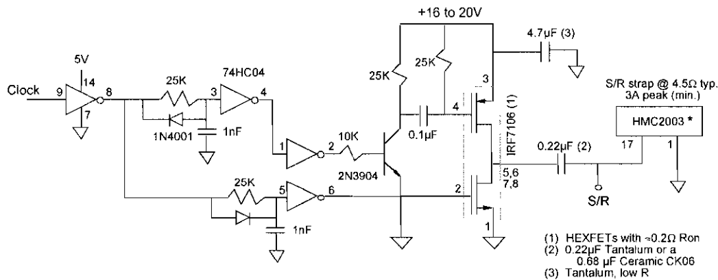
Figure 8—Single Clock Set/Reset Pulse Circuit (1001/1002)
