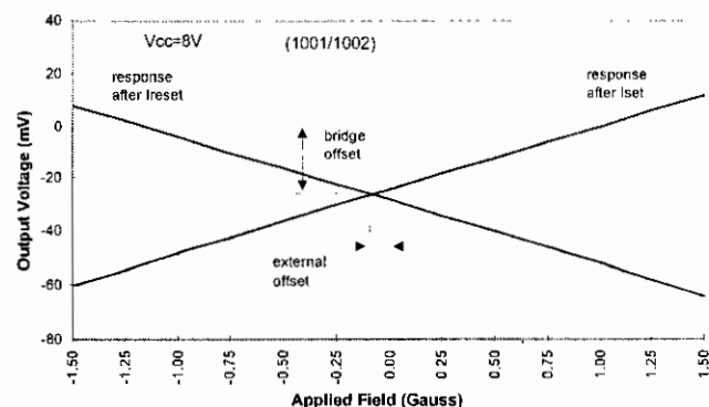
Figure 2—Output Voltage vs. Applied Magnetic Field
