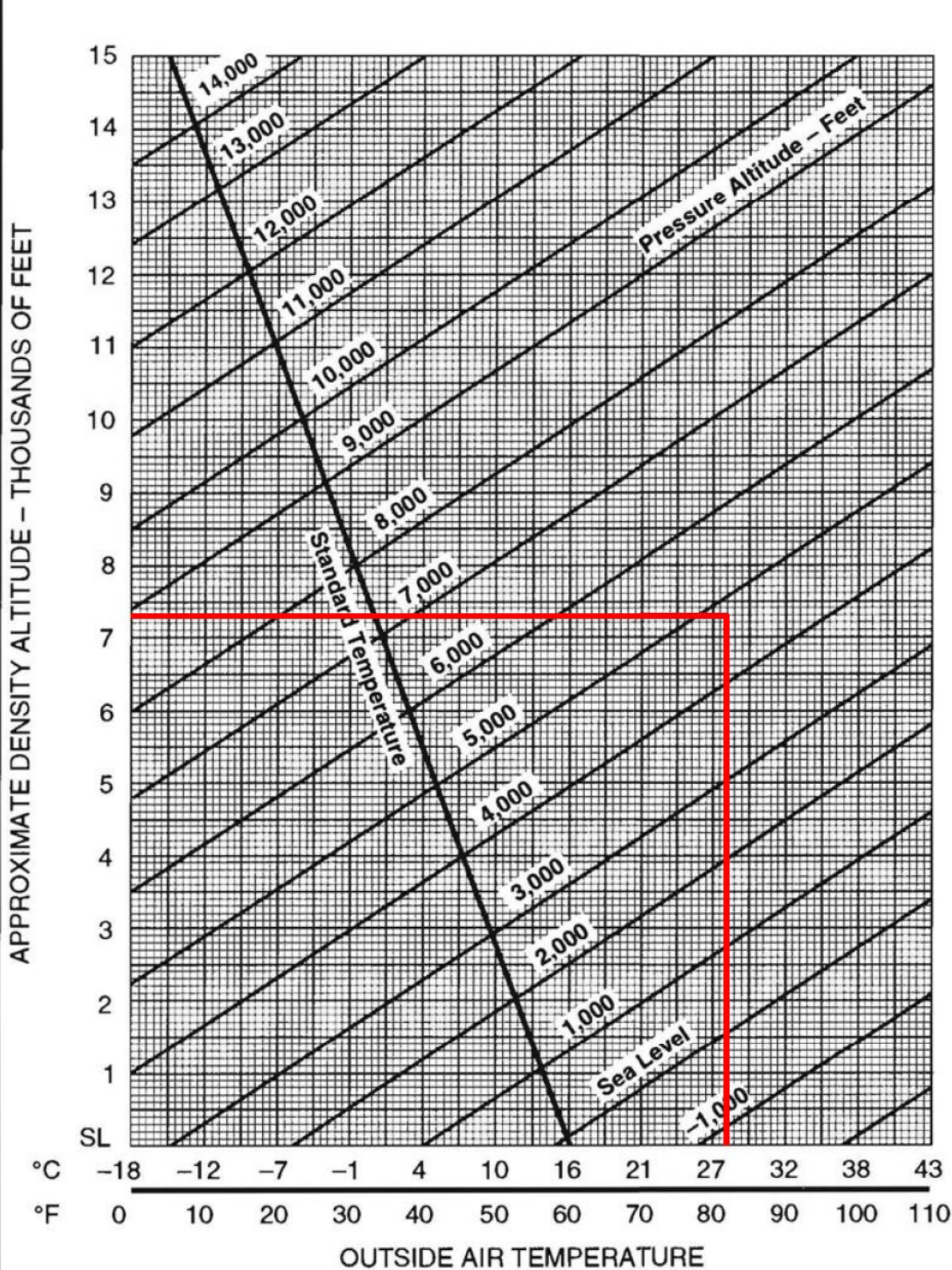
FIGURE 8.—Density Altitude Chart.
