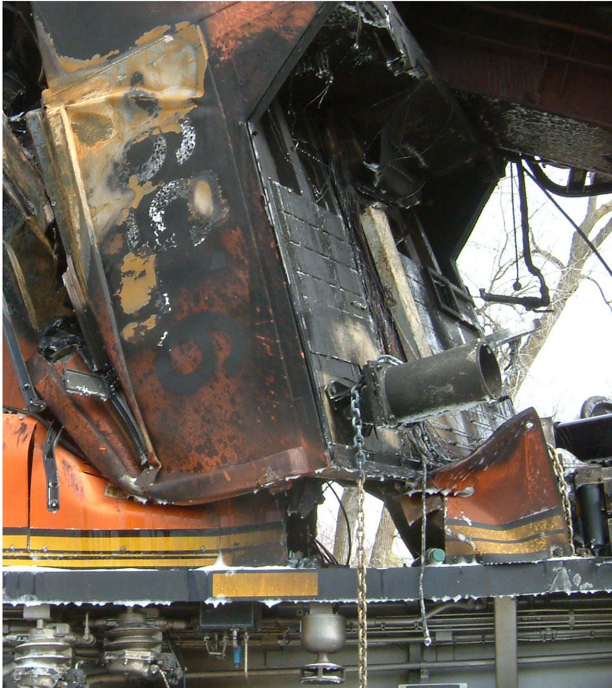
Exhibit 35-Photo Showing Rear Cylindrical Operators Cab Mounting Post Attached to Cab Flange on BNSF 9159
