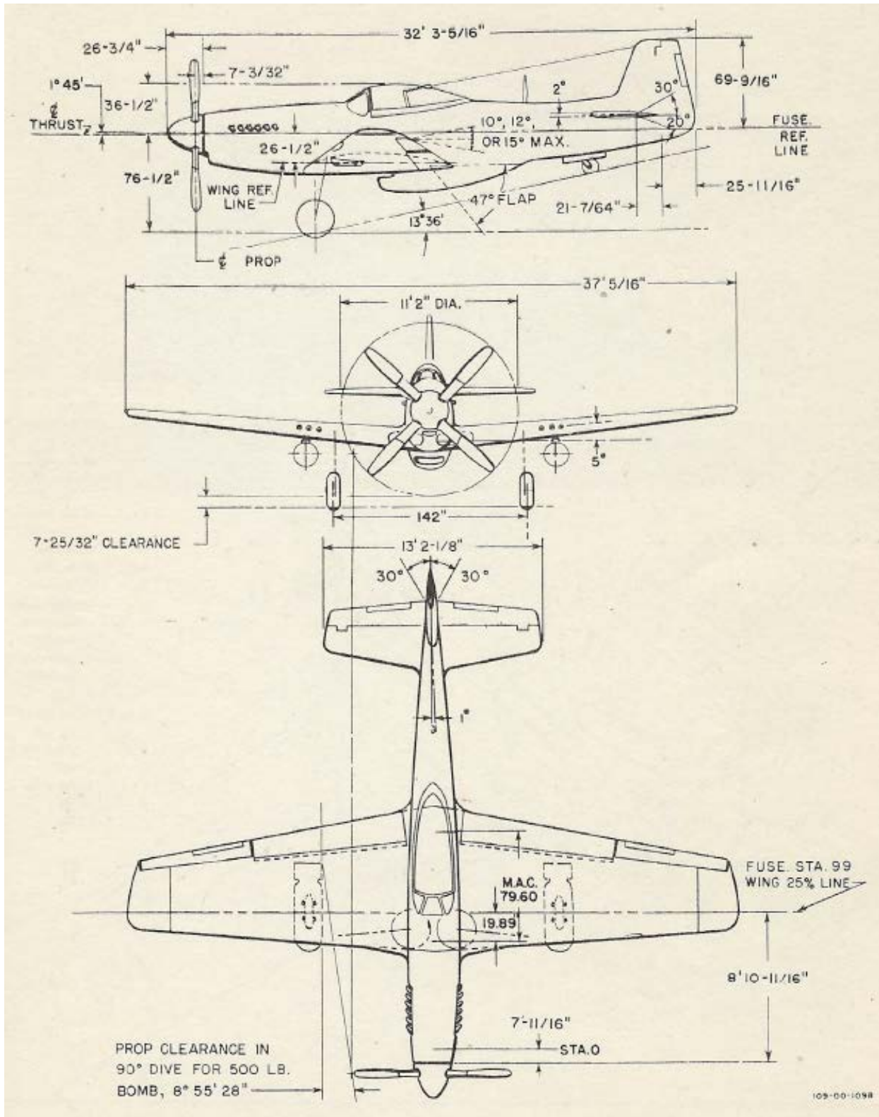
Figure 1 – Stock P-51D 3-view drawing
