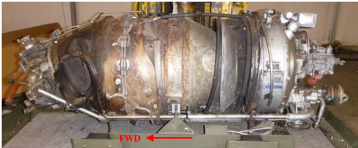
Figure 6 – PT6A-135A engine from N270PA
