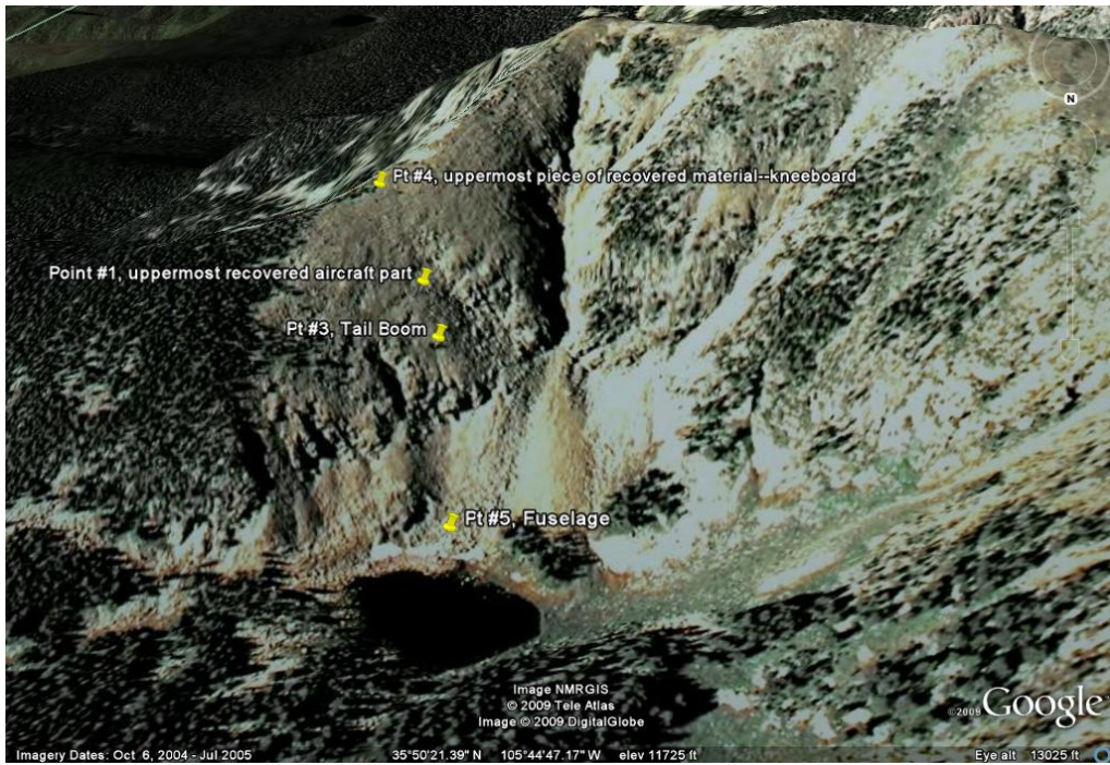
Figure 1 – Wreckage Disposition
