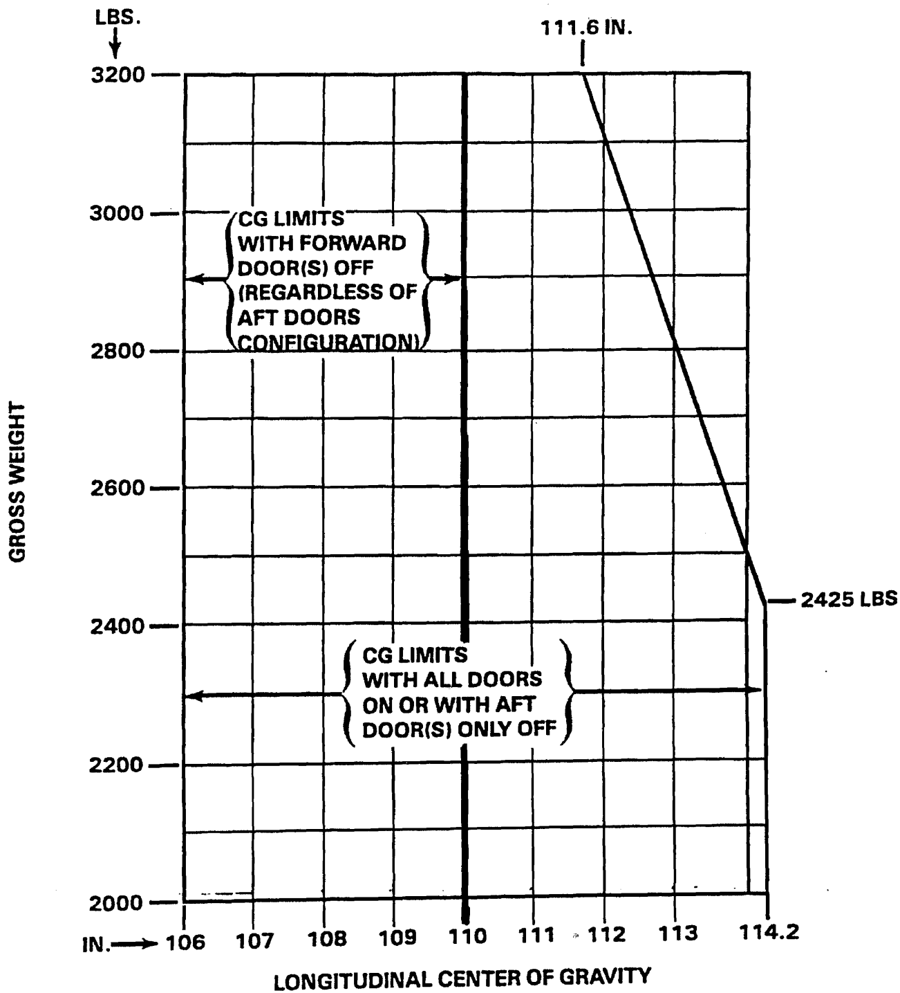
Figure 3-1. Center of gravity vs. Gross weight.
