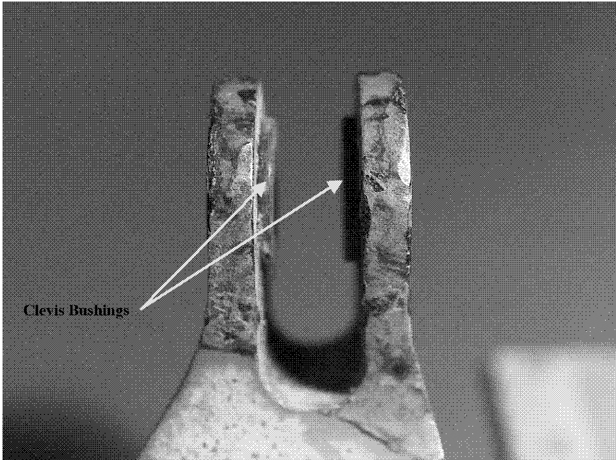
Photo 6: Close up of the R/H Control Tab Crank (clevis) Fitting. View looking aft. Note the contact damage on the forward face of each clevis lug.
