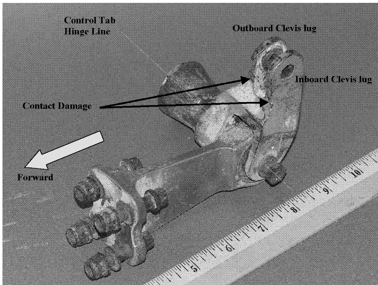
Photo 5: Digital photograph of the R/H Control Tab clevis fitting. View looking aft and outboard. Note the damage to the forward face of the clevis lugs.
