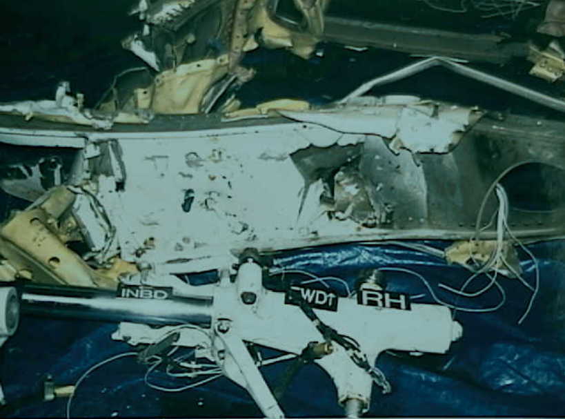
Airworthiness - Photo 8. View of right wing damage (view from forward looking aft). Note that the entire length of the wing spar was recovered. (NTSB-C3)
