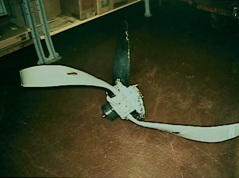
Airworthiness - Photo 24. View of all three propeller blades after removal from hub by investigators. Note "S" bending, chordwise scratching, and leading edge gouging. Also note two impressions in leading edge of blade no. 1 (denoted by arrow). (NTSB-CC)
