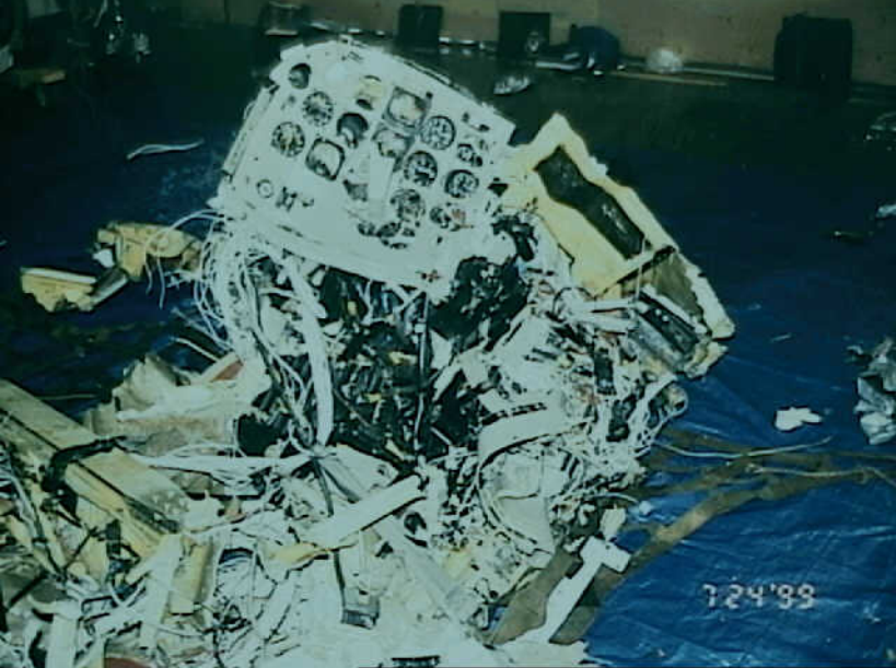
Airworthiness - Photo 1. View of the cockpit and cabin area. (NTSB-B2)
