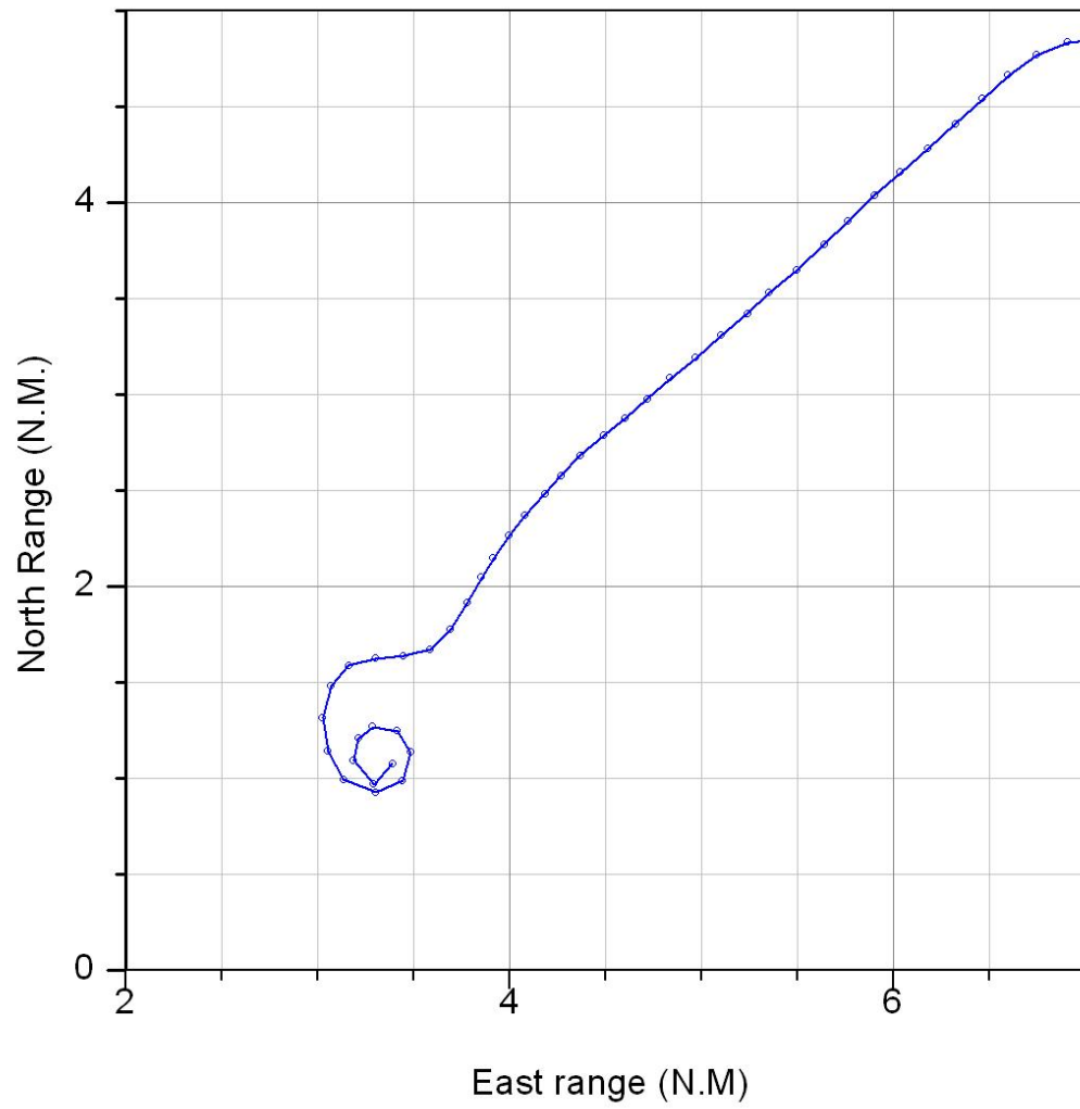
FAA Radar Data from KCAK ASR
