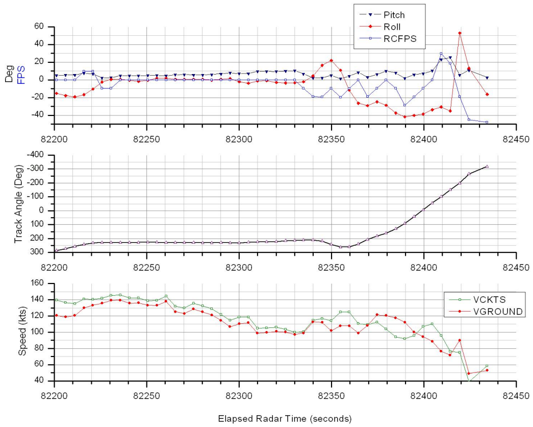
Radar data based calculated parameters
