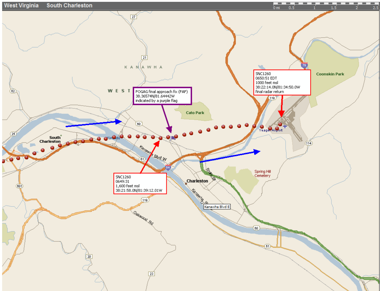
Figure 2 – Radar flight track of the final portion of flight of SNC1260 on May 5, 2017. Radar returns are indicated by red dots. Direction of flight is indicated by blue arrows. The FOGAG final approach fix is indicated by a purple flag.
