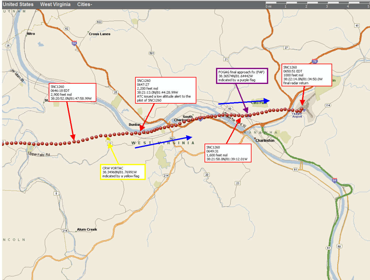
Figure 1 – Radar flight track of SNC1260 on May 5, 2017. Radar returns are indicated by red dots. The direction of flight is indicated by blue arrows. The CRW VORTAC location is indicated by yellow flag. The FOGAG final approach fix is indicated by a purple flag.
