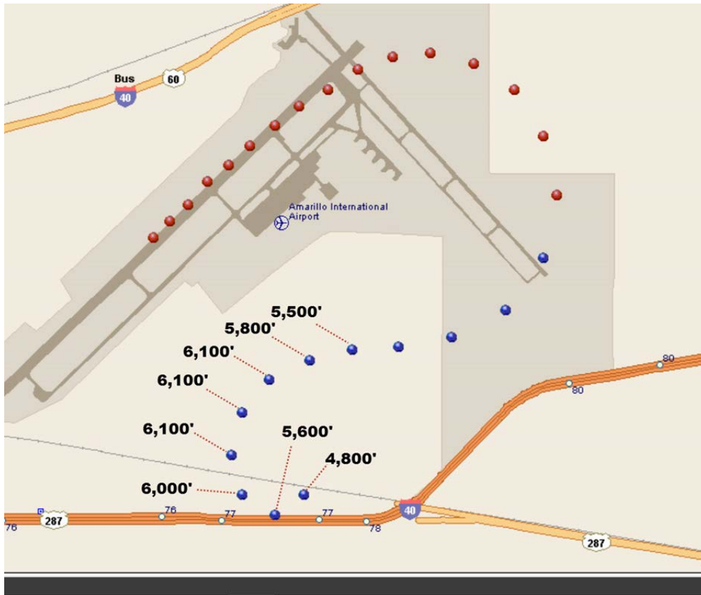
Figure 3 - Radar data illustrating the altitudes of the accident aircraft before the accident. The red target are the accident aircraft on the incorrect transponder code, the blue targets are the accident aircraft on the correct transponder code.
