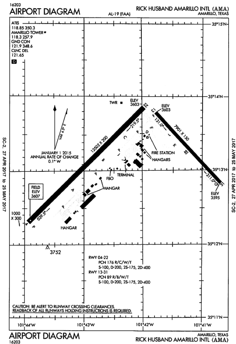
Figure 2 - AMA airport diagram effective April 27, 2017.
