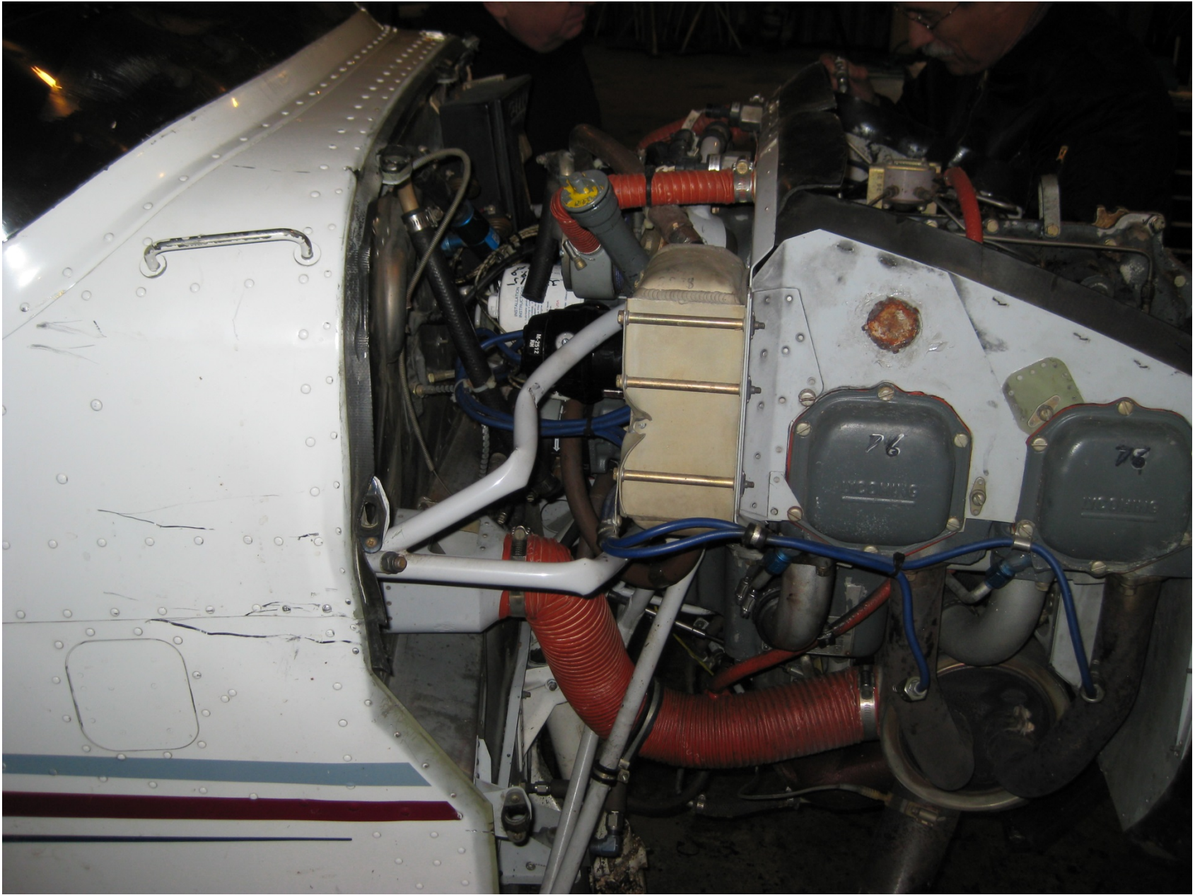
Photo 5 - View of buckled engine mounts
