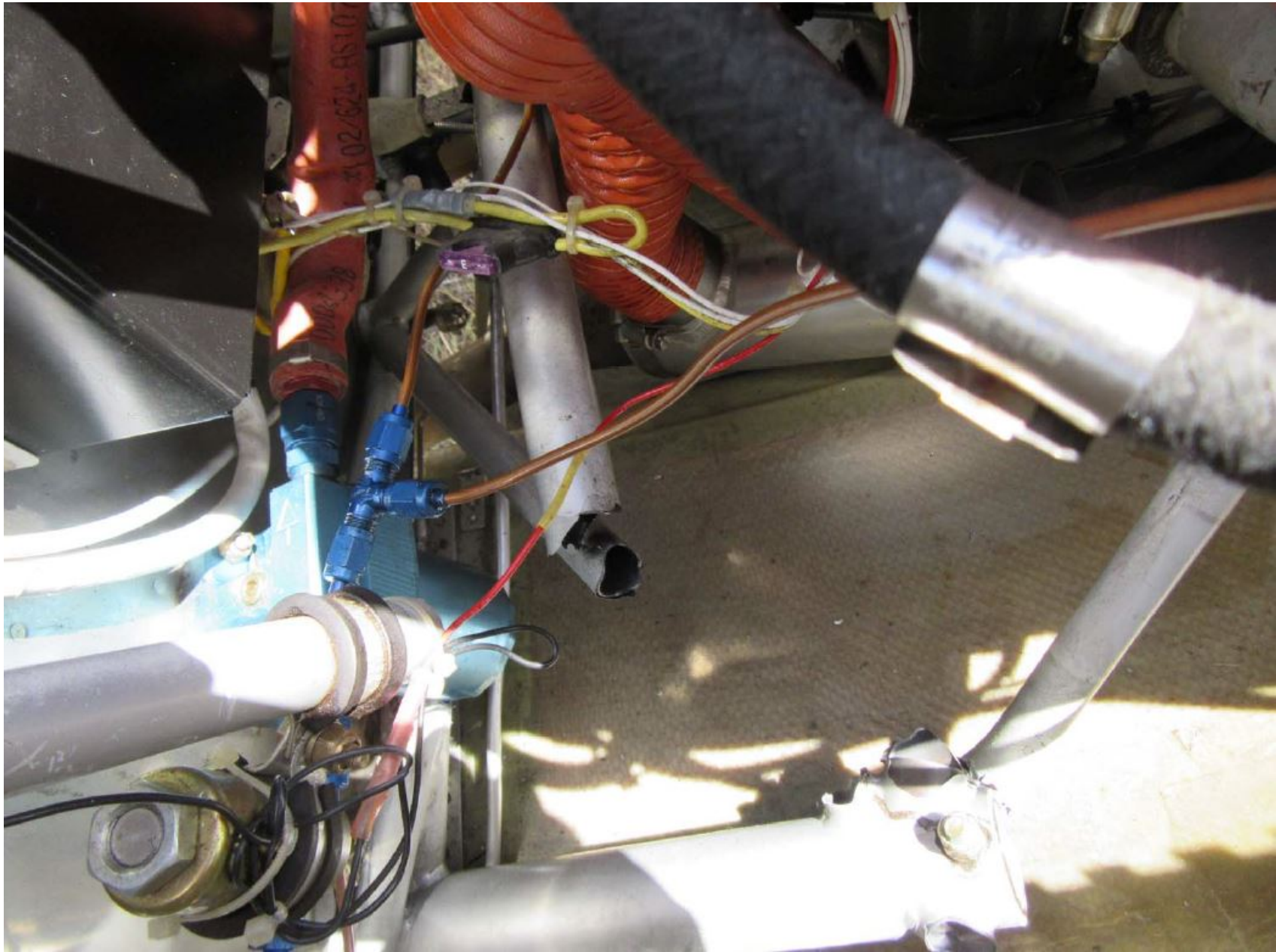
Photo 1 – View of damaged engine mount and truss (courtesy of the FAA)
