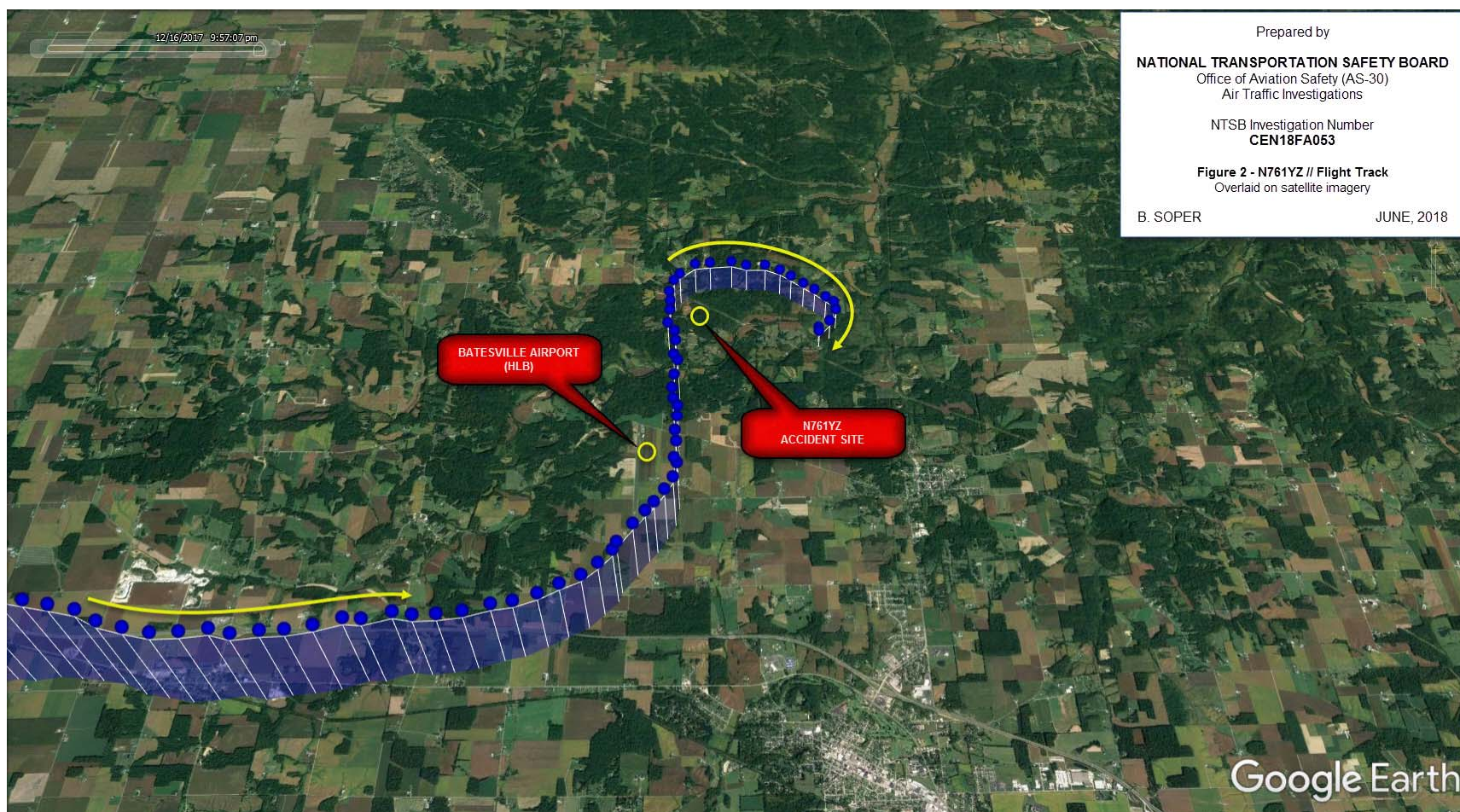
Figure 2. Radar flight track of N761YZ overlaid on satellite imagery with accident site and airport of intended emergency landing illustrated.
