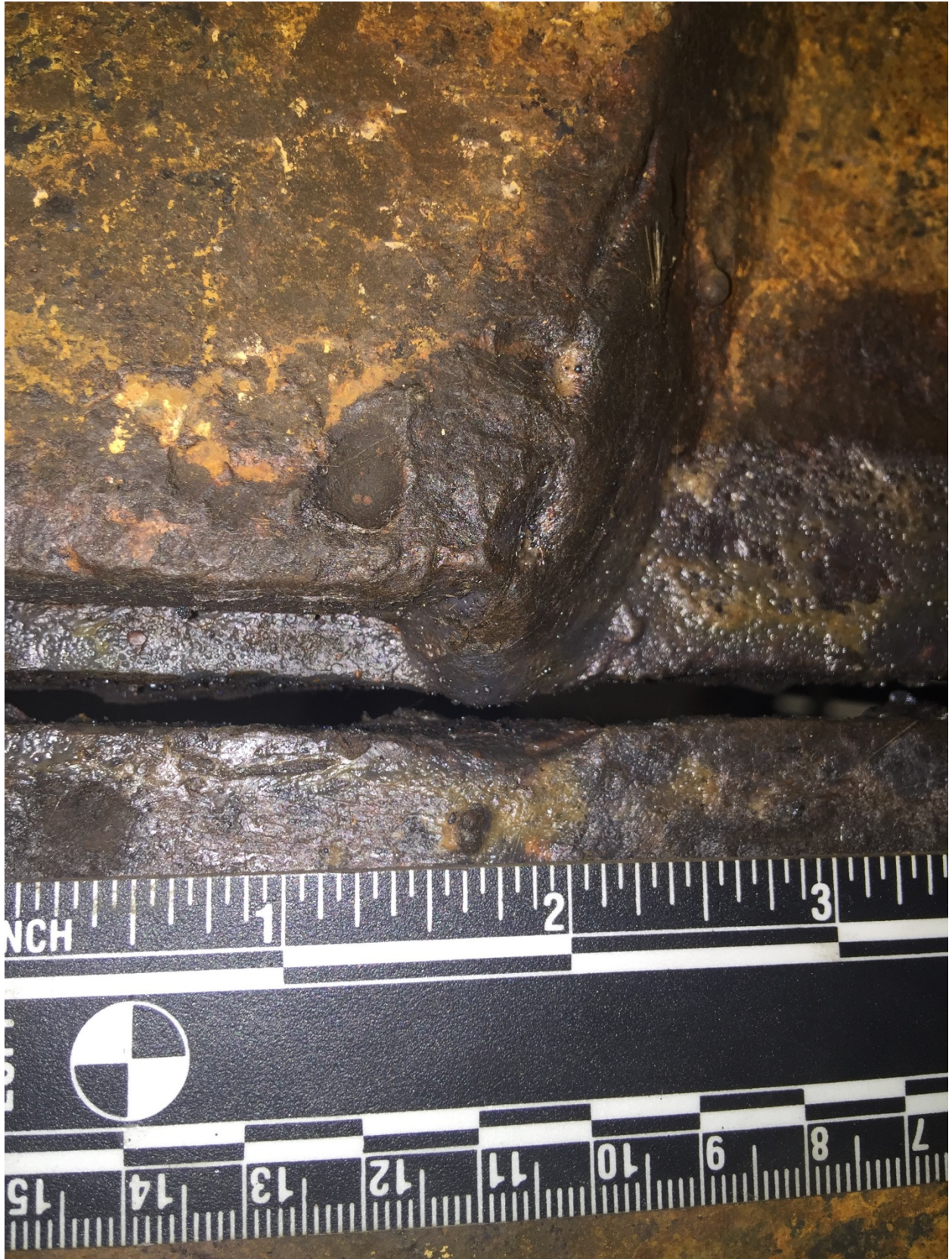
A-L cradle pad termination of A-6 fillet weld and tank shell crack initiation location, September 21, 2016.
