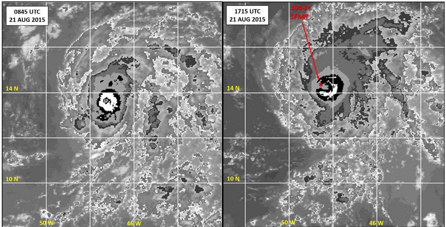
Figure 5. GOES-13 Infrared (BD-enhancement curve) satellite images at 0845 UTC and 1715 UTC 21 August 2015 when Danny was at its estimates peak intensity (left). Reconnaissance aircraft measured a SFMR surface wind value of 104 kt and a 700-mb flight-level wind of 111 kt (right) at the onset of the hurricane's rapid weakening trend. Images courtesy FNMOC, Monterey, CA.
