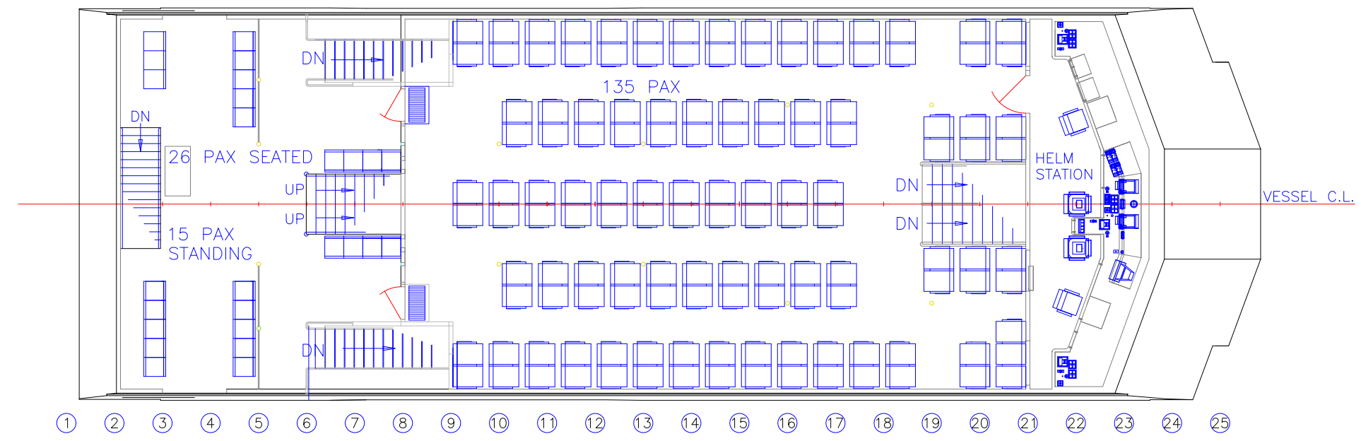
PLAN OF UPPER PASSENGER DECK
