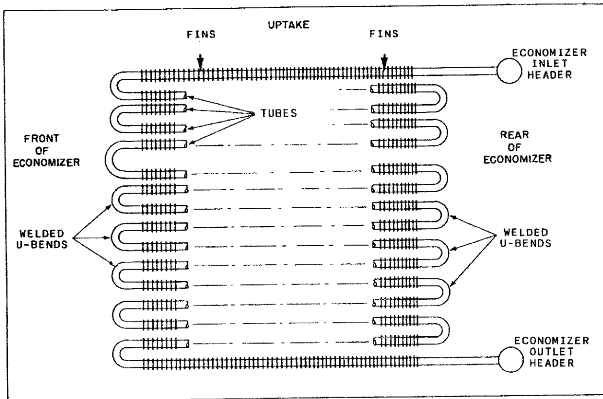
Figure 4-10.—Side view of an economizer.
