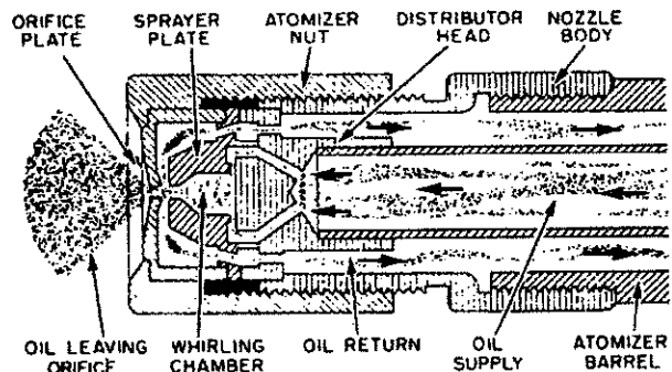
Figure 4-14.—Return-flow atomizer.
