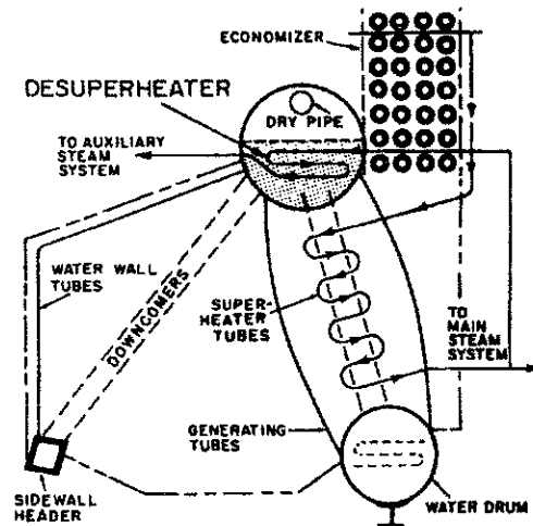
Figure 4-9.—Relative position of desuperheater tubes.
