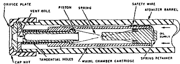
Figure 4-17.—Vented-plunger atomizer.
