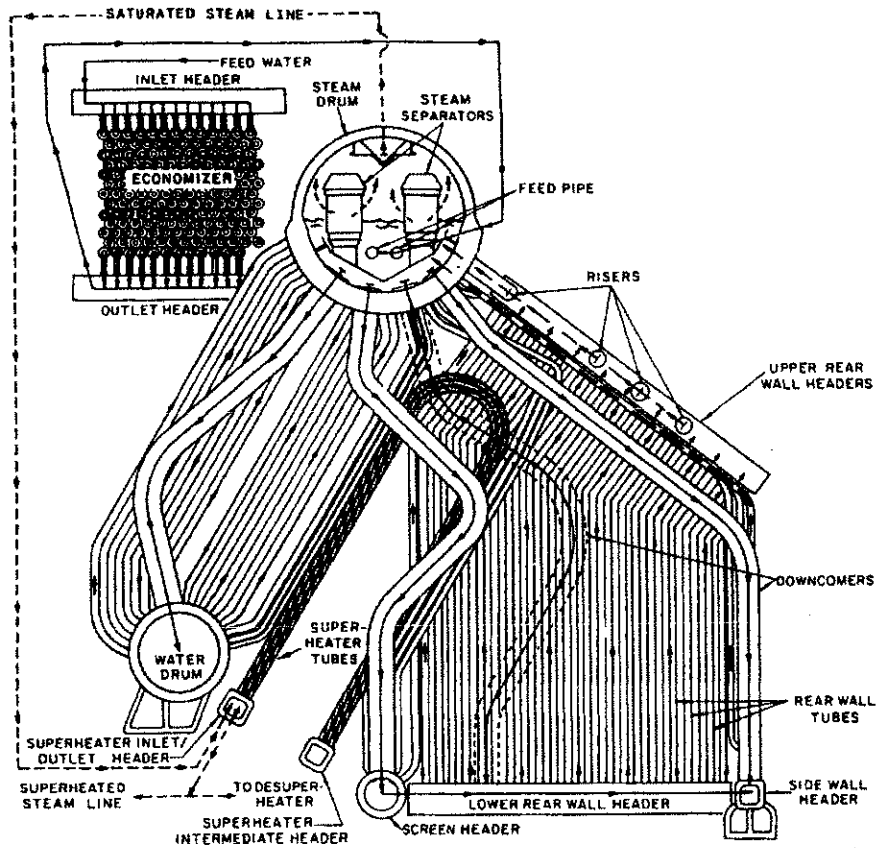
Figure 4-8.—Vertical superheater.
