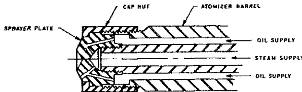
Figure 4-16.—Y-Jet steam atomizer.
