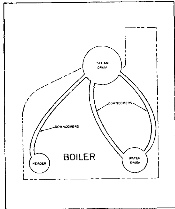
Figure 4-3.—Downcomer tubes.
