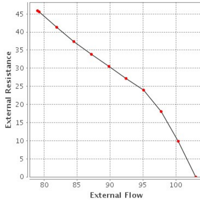
Auxiliary Pump Performance Chart
