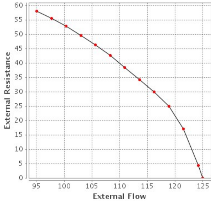
Auxiliary Pump Performance Chart
