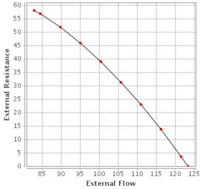
Auxiliary Pump Performance Chart
